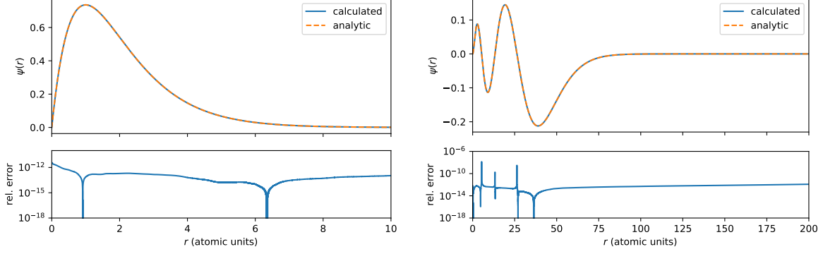
Figure 3.4: A comparison between the analytic and the calculated bound states for the ground state ( n = 1, l = 0 ) on the left, and n = 5, l = 1 on the right. The relative error of |\Psi_{\text{calc}} - \Psi_{\text{anal}}|/\Psi_{\text{anal}} is included underneath each plot. These were calculated with R_{\text{max}} = 1000, 300,000 points per grid, and R_{\text{min}} = 10^{-6} . The plots only show a portion of the r range of the wavefunctions so details can be seen.
