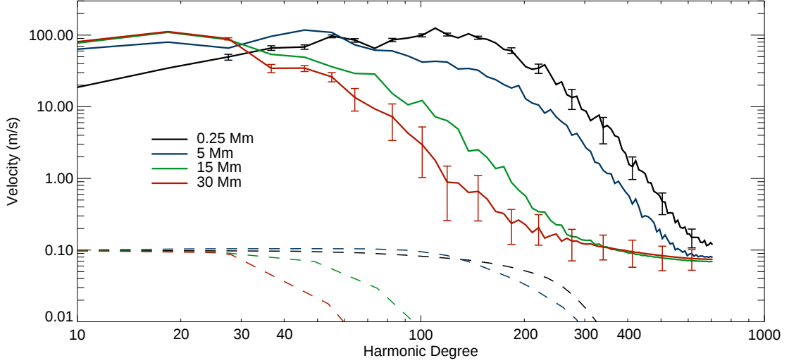
Figure 5.3: Spectrum of inversion results at a few depths as a function of harmonic degree. These results are from the central portion of analysis period A2 (see Table 2.1). Solid lines are the azimuthally integrated spectra of the horizontal velocity field, and color differentiates the central depth of the averaging kernel. Vertical error bars on the black and red curves indicate the 95% confidence interval, and those for the blue and green curves show similar trends. The dashed lines are the upper envelope of the averaging kernels for each depth and demonstrate the relative sensitivity of our inversion result to the true flows in the Sun. The sensitivity for every averaging kernel is unity at \ell = 0 by definition, but the dashed lines have been normalized to arbitrary values for visual clarity.
