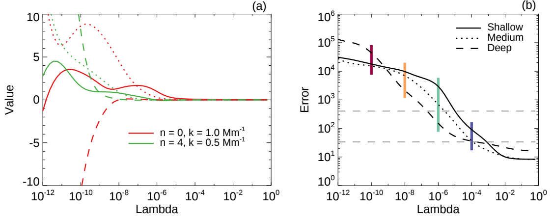
Figure 4.6: (a) Inversion coefficients for a shallow mode (red) and a deep mode (green) as a function of \lambda for the shallow target (solid lines), medium target (dotted lines), and deep target (dashed lines). (b) Estimated uncertainty on the inversion result as a function of \lambda for the three target depths. The horizontal dashed lines indicate the minimum and maximum of the uncertainties on all modes individually. Note the range with which the final uncertainty can be either amplified or reduced.
