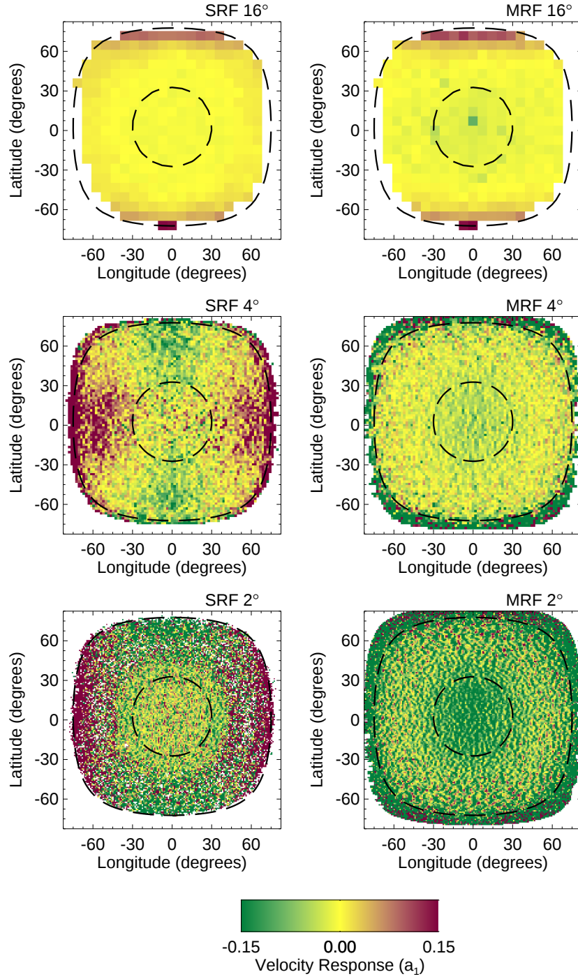
Figure 3.8: Velocity response for modes with lower turning points in the upper 16 Mm for 16° tiles, 4 Mm for 4° tiles, and 2 Mm for 2° tiles. The inner dashed circle is at 30° from disk center and the outer dashed line is at 75°. The SRF velocity response (left) has significantly higher spatial variability over the solar disk than the MRF method (right).
