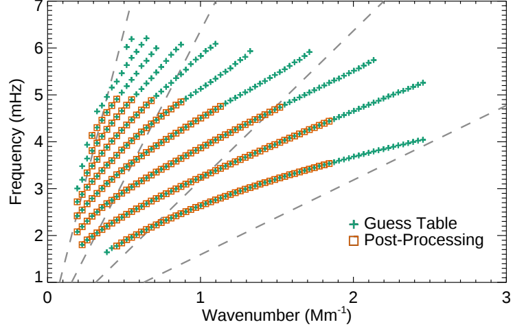
Figure 3.12: Comparison of the 16° tile guess table modeset (crosses) and the modeset after post-processing. The loss of high-phase-speed modes is largely due to the non-physical patterns seen in Figure 3.11.
