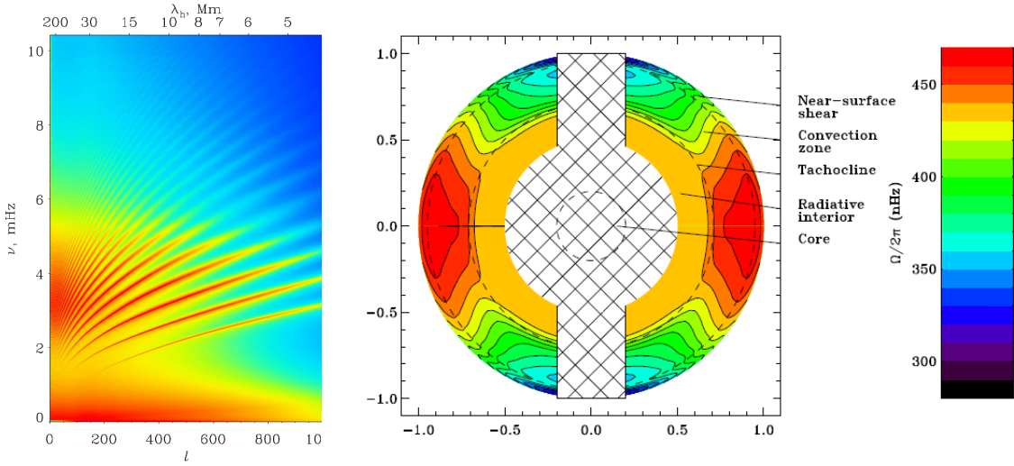
Figure 1.2: Left: Power spectrum of photospheric solar oscillations from SOHO/MDI. The ridges of power seen in this \nu - l (frequency vs. harmonic degree) diagram are created by the resonant waves of the solar interior. The lowest-frequency ridge corresponds to the surface gravity wave (the f -mode). Each higher ridge corresponds to pressure waves of increasing radial order ( p_1 , p_2 , etc.). Subtle variations in these ridges are measured and used to infer subsurface properties. Right: Rotation rate (angular velocity \Omega ) of the solar interior as a function of depth and latitude measured with global helioseismology (Howe 2009). These measurements reveal a set of distinct radial shells in the solar interior differentiated by rotational properties.
