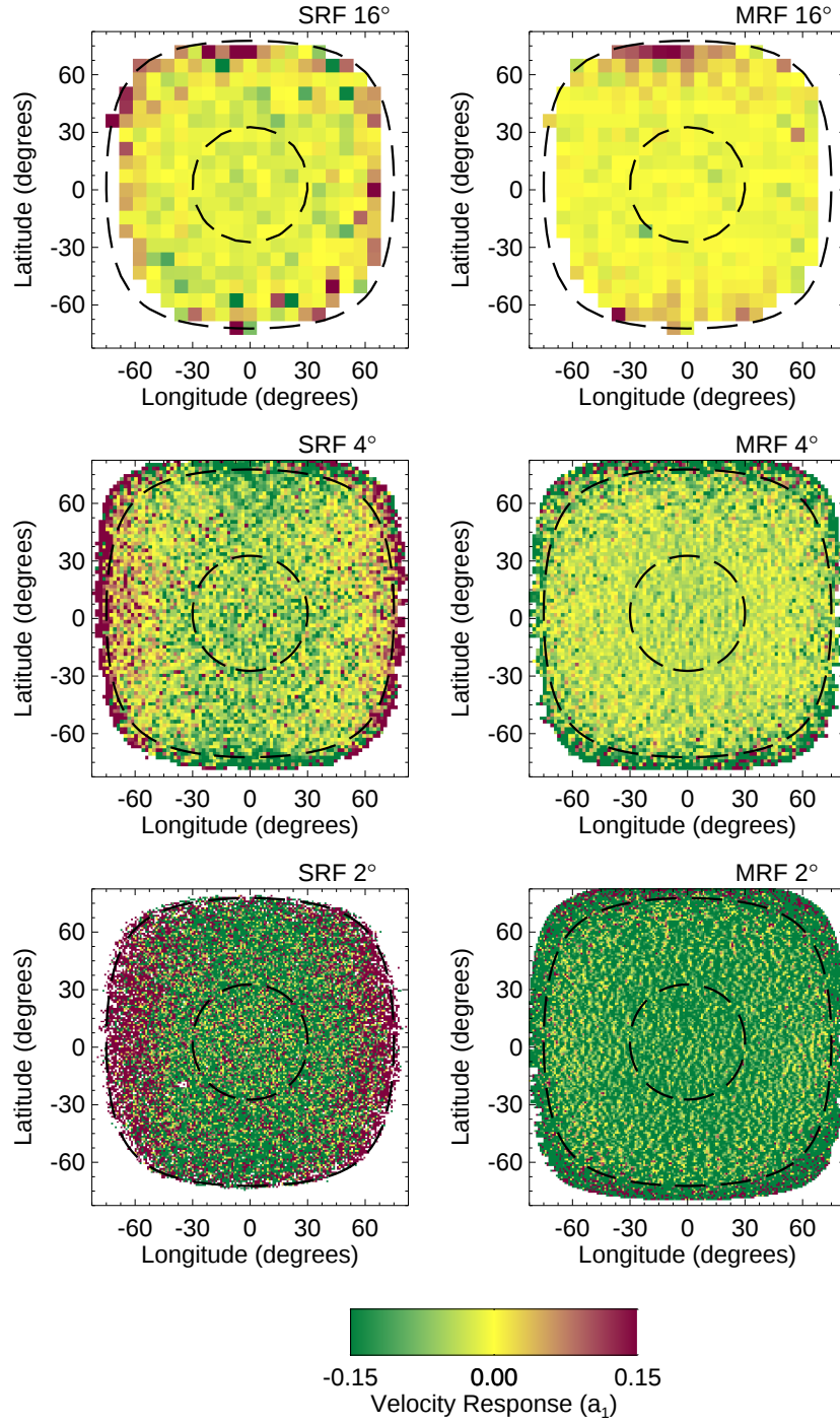
Figure 3.9: Velocity response for modes with lower turning points between 16 and 48 Mm for 16° tiles, between 4 and 12 Mm for 4°, and between 2 and 6 Mm for 2°. The inner dashed circle is at 30° from disk center and the outer dashed line is at 75°. Frequency shift measurements from deeper modes show less spatial variability over the solar disk for both the SRF method (left) and the MRF method (right).
