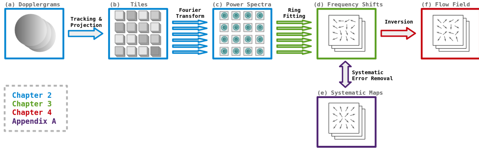
Figure 2.1: The steps involved in ring-diagram helioseismology. We can consider ring-diagram analysis as a sequence of processing steps that transform one data product into another. Here, the data products are in boxes and the processes are arrows. The data with which we start the process is a set of full-disk Dopplergrams (a). Dopplergram tiles (b) are created from this data set by tracking and projecting a mosaic of square regions. These tiles are then Fourier transformed and made into three-dimensional power spectra (c). The power spectra are then measured with a non-linear fitting code to produce frequency-shift measurements (d). Up to this point, each tracked and projected tile has been processed independently. The measured frequency shifts exhibit large-scale systematics as a function of disk position which can be measured and removed (e). The final step combines all of the frequency shifts in a single inversion to produce an estimate of the subsurface flow field (f). The colors of the boxes and arrows indicate the chapter of this thesis in which the topic appears in.
