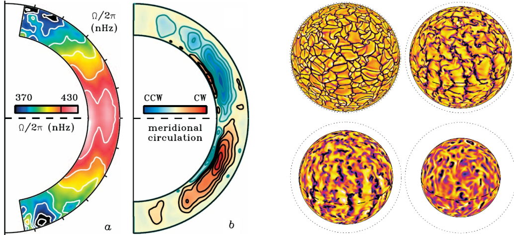
Figure 1.4: Results from a global simulation using the Anelastic Spherical Harmonic (ASH) code. Left: Panel (a) shows the temporally-averaged angular velocity as a function of latitude and depth, and panel (b) shows the average meridional circulation. This numerical simulation provided guidance on the global patterns of differential rotation and meridional circulation that might be expected in the Sun. Right: Vertical velocity at four different radii within the simulation. Dark colors indicate downflows and light colors indicate upflows. Near the surface, the cell-like structure of convection is clear. At depth, the effects of rotation can be seen with the vertical aligned convection cells (termed banana cells). Adapted from Miesch et al. (2008).
