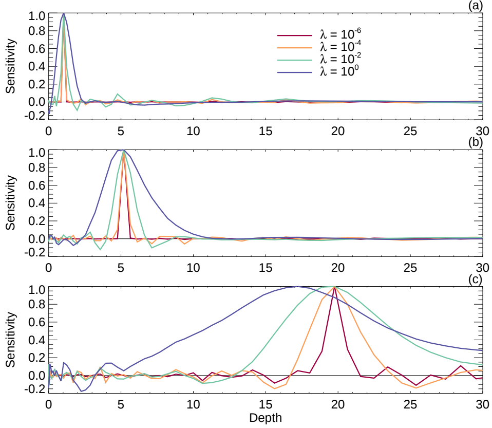
Figure 4.5: One-dimensional averaging kernels for a solar-like depth inversion with a target depth of 1 Mm (a), 5 Mm (b), and 20 Mm (c). The different colors show averaging kernels produces with different amounts of regularization. As the regularization parameter \lambda increases, the vertical localization of the averaging kernel suffers. For constant \lambda , the width of the averaging kernels gets larger for deeper target depths.
