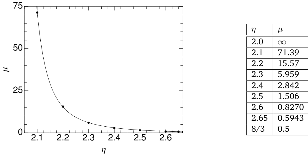
Figure 3.5: Some values of \mu as a function of \eta for 2 < \eta < 8/3 , found empirically by seeking, for each value of \eta , the solution that passes through the critical point. A numerical fit to these data is shown on the left, and a table of values is given to the right.
