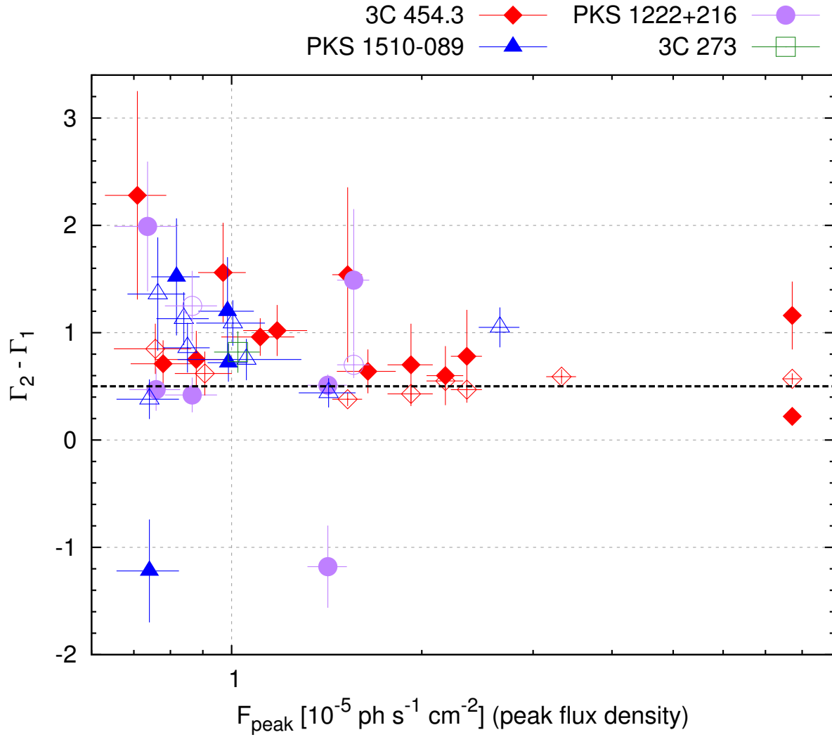
Figure 6.3: Distribution of the change in photon index \Delta\Gamma = \Gamma_2 - \Gamma_1 versus the peak flux F_{\text{peak}} ( 10^{-5} \text{ ph s}^{-1} \text{ cm}^{-2} ) of the flare, plotted for all identified spectral breaks in the 40 brightest Fermi gamma-ray flares. The shape and color of each point indicate the host blazar. Solid symbols indicate statistically significant primary and secondary breaks, whereas unfilled symbols indicate primary breaks that were not statistically significant. The dotted line denotes \Delta\Gamma = 0.5 , the value expected from a cooling break associated with radiative losses.
