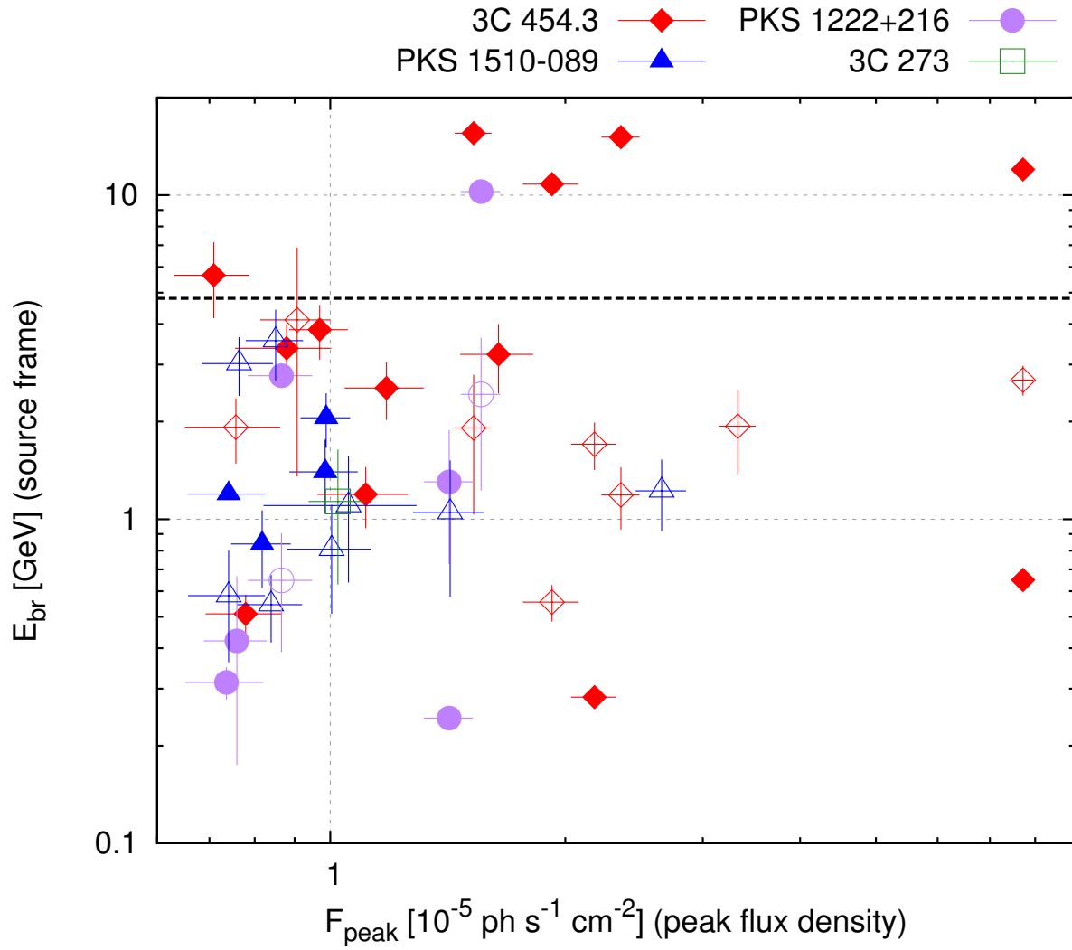
Figure 6.2: Distribution of the source-frame break energy E_{br} (GeV) vs. the peak flux F_{peak} ( 10^{-5} \text{ ph s}^{-1} \text{ cm}^{-2} ) of the flare, plotted for all identified spectral breaks in the top 40 Fermi gamma-ray flares. The shape and color of each point indicate the host blazar. Solid symbols indicate statistically significant primary and secondary breaks, whereas unfilled symbols indicate primary breaks that were not statistically significant.
