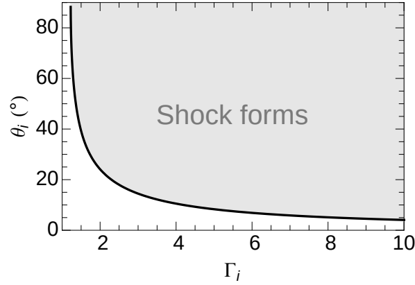
Figure 5.1: Minimum angle of impact necessary to produce a shock, plotted as a function of the initial bulk Lorentz factor of the flow at the point of impact. The shaded region corresponds to combinations of angle and Lorentz factor that will result in a shock forming.
