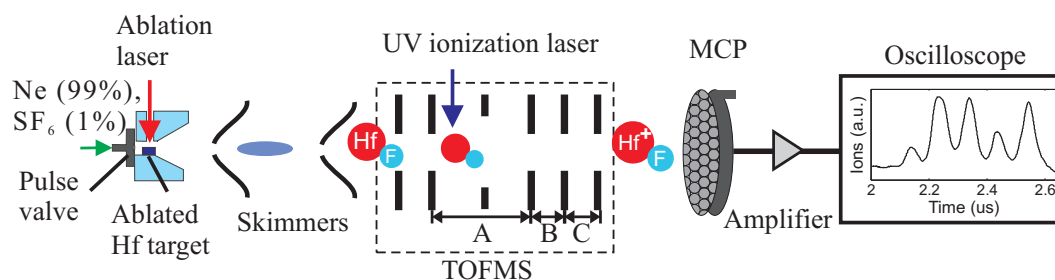
Figure 2.1: Schematic of the resonance-enhanced multiphoton ionization (REMPI) experiment.
