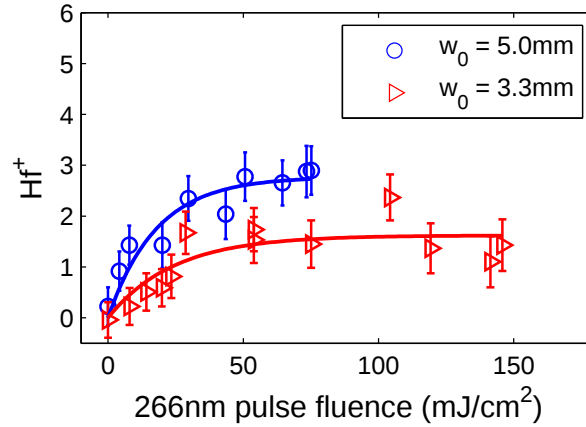
Figure 6.9: Saturation of the 1+1' photodissociation transition with 266 nm laser pulse energy. Two different beam waists were used for the 266 nm laser: (blue circles) w_0 = 5.0 \text{ mm} and (red triangles) w_0 = 3.3 \text{ mm} . The saturation behavior is fit to a single exponential A(1 - \exp(-F/F_S)) . The smaller exponential amplitude for the smaller beam waist is due to a less complete spatial overlap between the 266 nm laser and the ion cloud.
