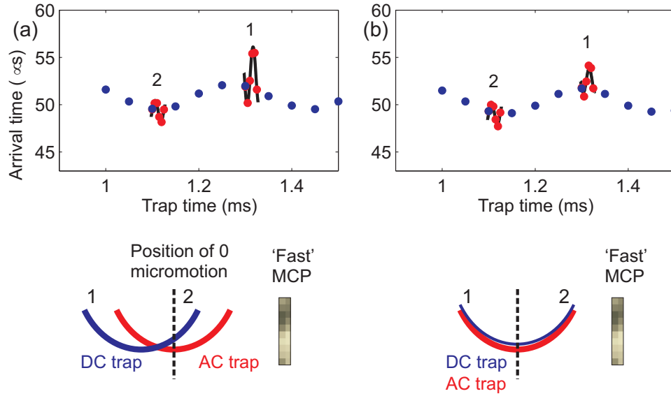
Figure 4.8: Plots of micromotion (red data points, 1 period = 25 \mu\text{s} ) at different trap positions (secular motion shown in blue): at position '1' ('2'), the ions are displaced farther from (nearest towards) the 'fast' MCP detector. (a) A dipolar patch field has displaced the ions away from the center of the harmonic pseudopotential formed by the RF voltages (denoted as 'AC trap'), so the micromotion tends to be larger at position '1' than at '2'. (b) When the dipolar patch field is nulled out, the micromotion is equal at both positions '1' and '2'.
