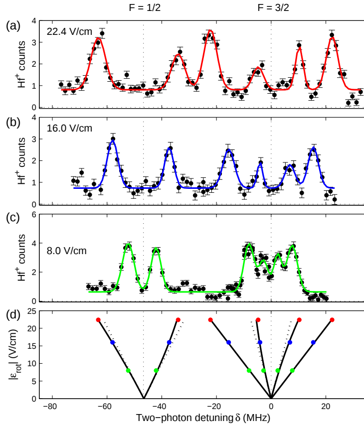
Figure 7.9: Stark spectroscopy of the ^3\Delta_1(\nu = 0, J = 1) state with a rotating bias field of (a) 22.4 V/cm, (b) 16.0 V/cm and (c) 8.0 V/cm/ (d) The Stark-shifted peak positions are plotted as a function of rotating electric field magnitude as colored dots. The dashed lines are the linear Stark shifts from Eq. (7.21) and the solid lines are the Stark shifts including perturbation effects as described in Eq. (7.23).
