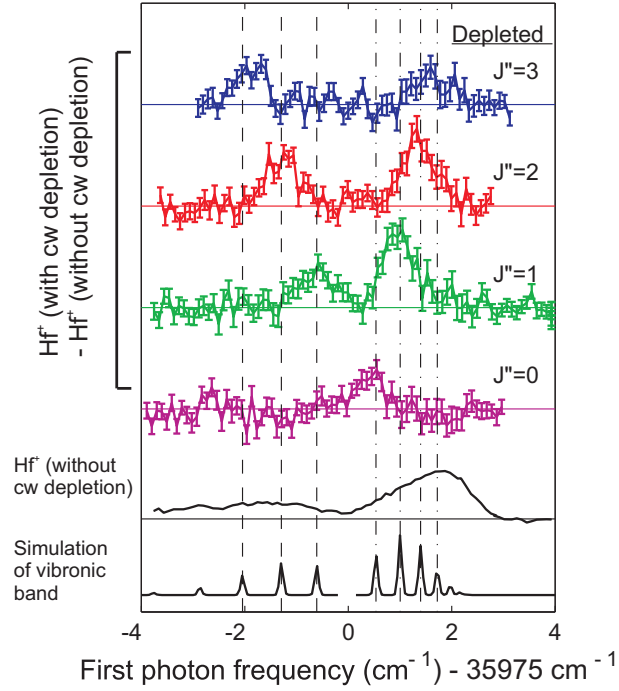
Figure 6.7: Depletion spectroscopy of the \Omega' = 0 \leftarrow {}^1\Sigma^+ vibronic band at 35975 \text{ cm}^{-1} (shown as the unresolved, thick black line in the second lowest panel). To resolve the individual rotational lines, the vibronic band is scanned over in the presence of a depletion laser driving a particular rotational transition of the {}^1\Pi_1 \leftarrow {}^1\Sigma^+ band, and the difference in Hf^+ with and without the depletion laser is plotted as the colored lines with error bars. The thin black line (bottom panel) denotes the simulated vibronic band with its R branch on the right (dot-dashed vertical lines) and P branch on the left (dashed vertical lines).
