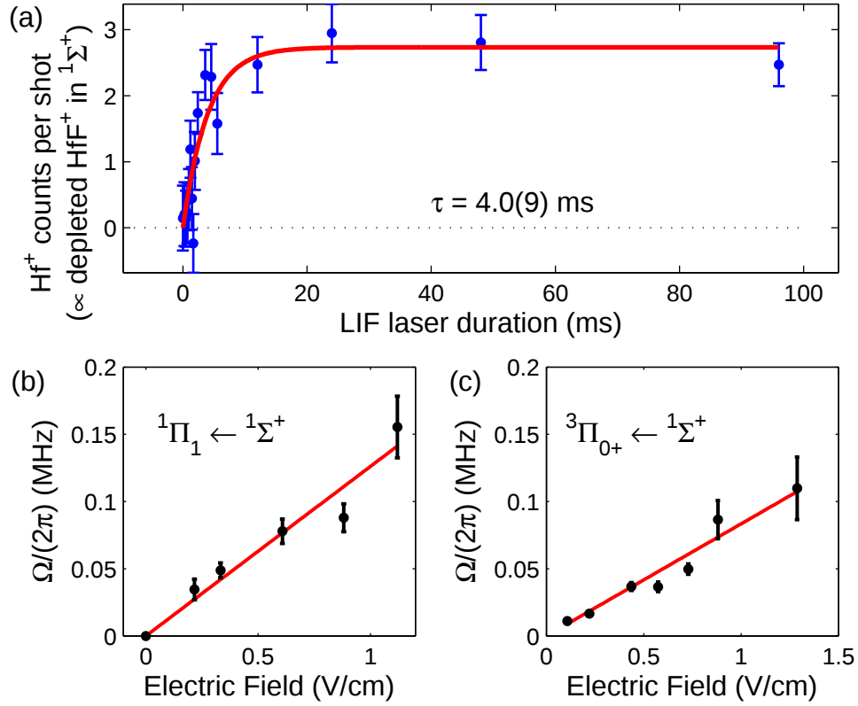
Figure 7.3: (a) Number of HfF + ions transferred out of the 1\Sigma^+ state (detected as the difference in dissociated Hf + counts with and without the LIF laser) as a function of LIF laser duration, where the LIF laser is tuned to resonance with the 1\Pi_1(\nu' = 0, J' = 1) \leftarrow 1\Sigma^+(\nu'' = 0, J'' = 1) transition. For this data, the Doppler width (one-photon detuning \Delta ) was anomalously large at 120 MHz. Nevertheless, the decay time constant of 4.0(9) ms, which is measured for a particular LIF laser intensity of 0.49 mW/cm 2 , can be converted to a LIF laser Rabi frequency of (2\pi)0.078(9) MHz and plotted as a single point in (b). (b) Plot of Rabi frequency versus laser electric field for the 1\Pi_1(\nu' = 0, J' = 1) \leftarrow 1\Sigma^+(\nu'' = 0, J'' = 1) LIF transition. The slope gives the rovibronic transition dipole moment to be 0.098(13) e a_0 . (c) Plot of Rabi frequency versus laser electric field for the 3\Pi_{0+}(\nu' = 1, J' = 1) \leftarrow 1\Sigma^+(\nu'' = 0, J'' = 0) transition. The slope gives the rovibronic transition dipole moment to be 0.065(9) e a_0 .
