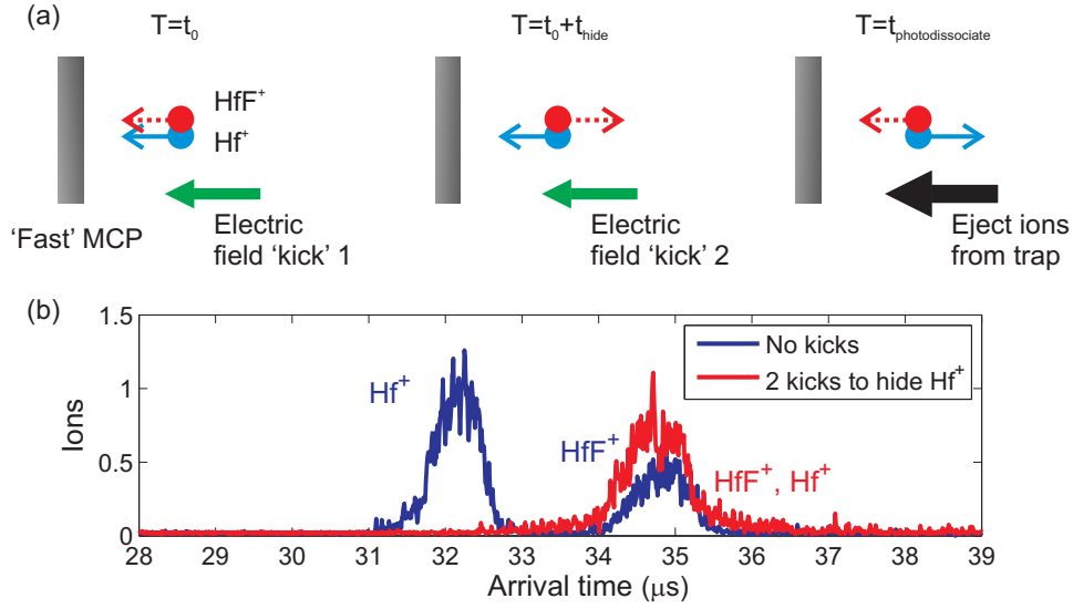
Figure 6.5: Hiding aboriginal \text{Hf}^+ ions. (a) A pair of velocity ‘kicks’ is applied to the ions at times t_0 and t_0 + t_{\text{hide}} , which are chosen such that the \text{Hf}^+ and \text{HfF}^+ ions are moving in phase and out of phase relative to each other, respectively. In this way, the \text{HfF}^+ ions remain stationary whereas the \text{Hf}^+ ions oscillate with an even larger velocity after the second ‘kick’. When the photodissociation lasers fire, the \text{Hf}^+ ions should be moving away from the detector, so that they eventually arrive the MCP at the same time as the heavier \text{HfF}^+ ions. (b) Two oscilloscope traces depicting the arrival of \text{Hf}^+ and \text{HfF}^+ with (red) and without (blue) the pair of ‘kicks’. Without the ‘kicks’, the bump at earlier (later) time indicates the arrival of \text{Hf}^+ ( \text{HfF}^+ ). With the ‘kicks’, both ion species arrive at the same time. This data is recorded with the \text{Hf}^+ and \text{HfF}^+ ions created by ionizing both neutral Hf atoms and HfF molecules.
