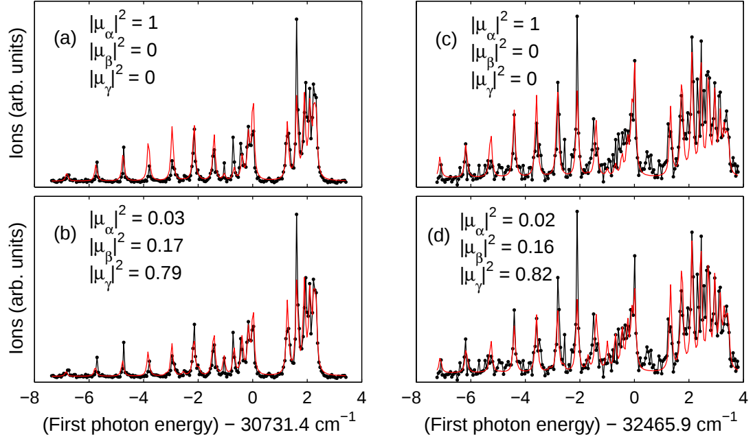
Figure 2.5: Contour fits (red) to the \Omega' = 3/2 \leftarrow X^2\Delta_{3/2} {30.73} and {32.47} bands (data shown as connected black dots). In (a, c), the contour fits are constrained to use Hönl-London expressions for the rotational line strengths, which are shown here to be inadequate for a good description of the observed line intensities, especially for those in the Q branch. In (b, d), the contour fits are allowed to take into account possible interference effects between parallel and perpendicular transition moments. In both cases, \mu_\gamma dominates over the other transition dipole matrix elements, indicating that the nominal \Omega' = 3/2 upper states in both cases appear to possess an admixture from nearby \Omega' = 1/2 states.
