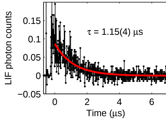
Figure 7.2: Lifetime of the ^1\Pi_1(\nu' = 0) state measured using LIF.
