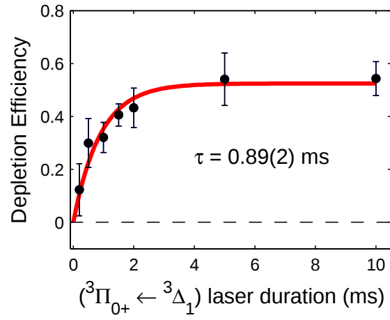
Figure 7.4: Depletion efficiency of the ^3\Delta_1 HfF ^+ ions as a function of the 986.4 nm side-depletion laser duration, where the 986.4 nm laser of intensity 70 mW/cm ^2 is tuned to resonance with the ^3\Pi_{0+}(\nu' = 1, J' = 1) \leftarrow ^3\Delta_1(\nu = 0, J = 1) transition. The decay time constant of 0.89(2) ms implies a rovibronic dipole matrix element of 0.04(1) e a_0 .
