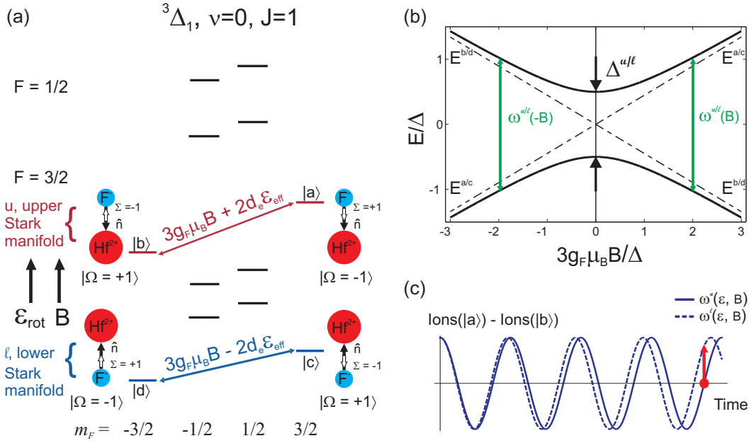
Figure 8.1: (a) (Reproduced from Fig. 1.5) \text{HfF}^+ energy levels in the ^3\Delta_1, \nu = 0, J = 1 state in the presence of an external electric and magnetic field, where the eEDM-sensitive transitions are between states |a\rangle and |b\rangle and between states |c\rangle and |d\rangle . (b) In the presence of a rotating quantization axis, |a\rangle and |b\rangle (similarly, |c\rangle and |d\rangle ) are coupled to each other and form an avoided crossing as a function of magnetic field. At the center of the avoided crossing (i.e. no magnetic field), the eigenstates are equal superpositions of the stretch states of the same Stark manifold, e.g. \{|0\rangle, |1\rangle = (|a\rangle \pm |b\rangle)/\sqrt{2}\} for the upper Stark pair. The vertical green arrows denote the eEDM-sensitive transition frequencies. (c) Ramsey fringes measured for the upper (solid) and lower (dashed) Stark manifolds. The eEDM signal is proportional to the amount by which the Ramsey fringe moves when sitting on the side of a fringe.
