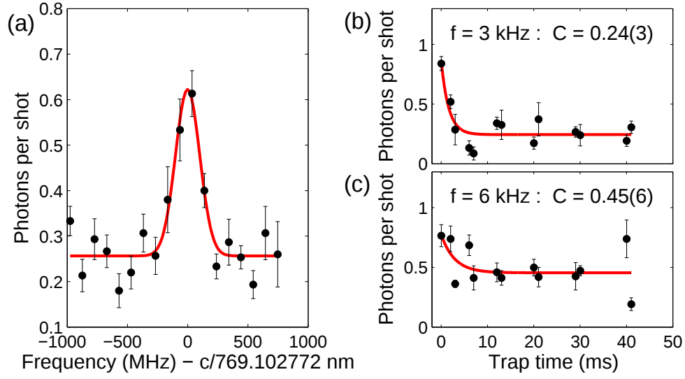
Figure 5.3: (a) Frequency scan of the ^1\Pi_1 \leftarrow ^1\Sigma^+(0,0) Q(1) transition, taken by performing LIF on ions that have been trapped for 2 ms. (b) Plot of LIF signal as a function of trap duration for a 3 kHz trap. The signal is fit to a decaying exponential with offset C . (c) Plot of LIF signal as a function of trap duration for a 6 kHz trap. The tighter trap in (c) yields a larger LIF signal C at long times compared to the weaker trap in (b).
