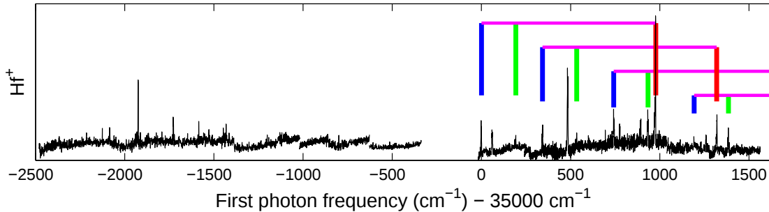
Figure 6.6: REMP spectroscopy of \text{HfF}^+ transitions at 32500\text{--}36500\text{ cm}^{-1} , detected by photodissociating \text{HfF}^+ into \text{Hf}^+ and \text{F} . The gap in the spectrum is due to Wood's anomaly of the laser grating that causes a loss in laser intensity. Transitions that have been identified as originating from the ^1\Sigma^+(\nu''=0) , ^1\Sigma^+(\nu''=1) and ^3\Delta_1(\nu''=0) lower states to excited states at > 30000\text{ cm}^{-1} are denoted by red, green and blue vertical lines, respectively. Vertical lines connected by a horizontal magenta line belong to transitions terminating on the same upper vibronic state.
