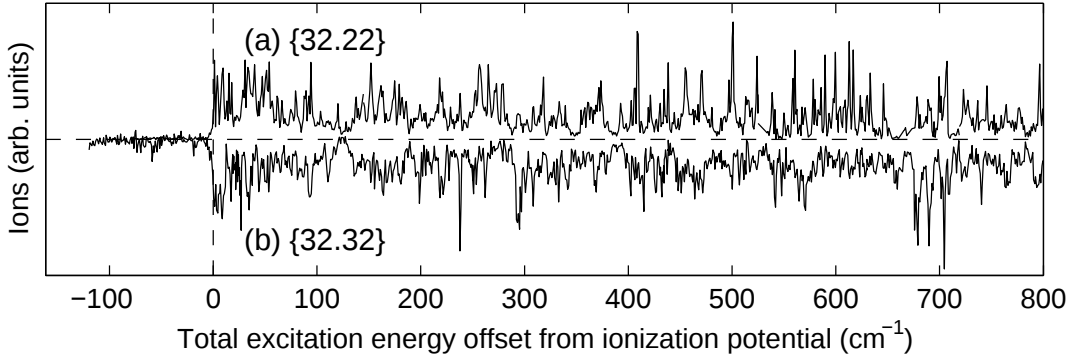
Figure 2.8: OODR autoionization spectra measured by tuning the first photon to access a particular excited rotational state ( J' = 1/2(a) ) using the vibronic bands (a) \{32.22\} and (b) \{32.32\} (ion signal inverted for clarity), then scanning the second photon to map out the spectrum of autoionizing Rydberg states accessible from that intermediate state. Each case gives a unique set of autoionization resonances, suggesting that the ionic core of the autoionizing Rydberg state differs between the two cases.
