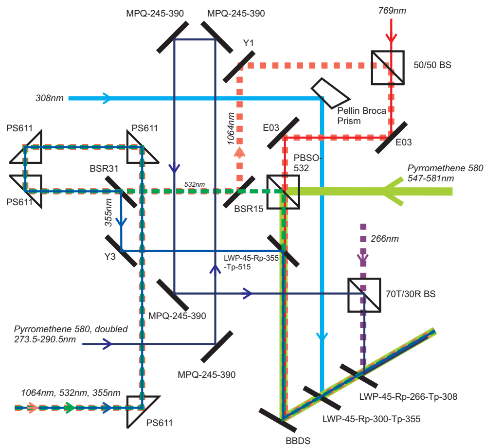
Figure 6.3: Layout of optics used to overlap 8 laser beams (wavelengths in italics ) in a search for photodissociation transitions. Table 6.1 gives a list of specifications for most of the optics shown.
