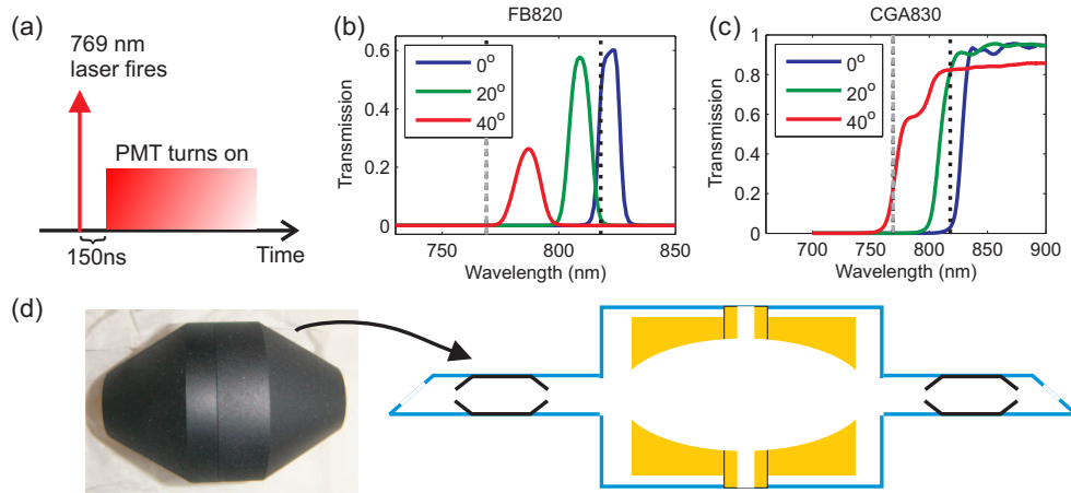
Figure 5.2: (a) Time gating of the PMT to reduce the detection of scattered light from the 769 nm excitation laser. (b) Plots of the bandpass filter FB820 transmission versus wavelength for different angles of incidence. (c) Plots of the colored glass alternative long-pass dichroic filter CGA830 transmission versus wavelength for different angles of incidence. In both (b) and (c), the gray dashed lines denote the excitation laser wavelength at 769 nm, at which scattered light is the strongest and needs to be suppressed most aggressively. The dotted black lines denote the fluorescence wavelength at 818 nm, at which the filters need to have high transmission for efficient fluorescence collection. (d) Photograph of a light baffle, which is placed in between the ion trap and Brewster window to reduce scattered light.
