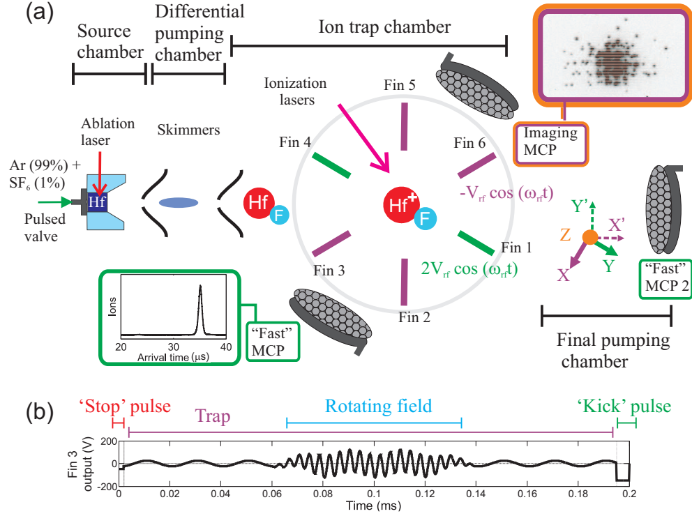
Figure 4.4: (a) Bird's eye view schematic of the HfF + source and ion trap setup. In the ion trap chamber, HfF + are formed in-situ by autoionization, trapped, and then ejected onto one of the three diagnostic MCPs, which allows us to detect both the ion number and motion in-trap. The top and bottom end cap electrodes are not shown. (b) Voltage output on one of the radial fin electrodes (fin 3).
