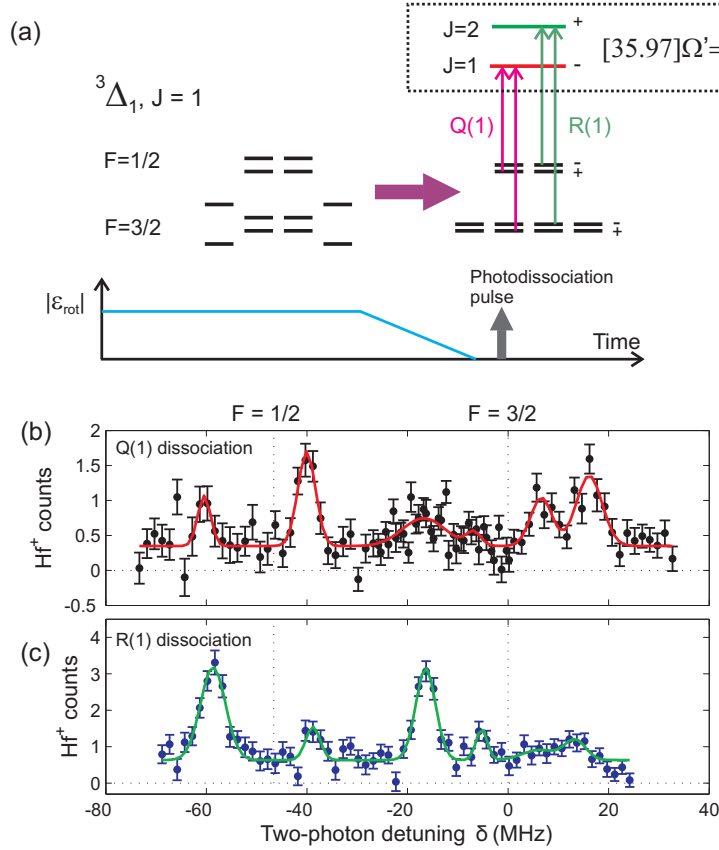
Figure 7.8: (a) Spectroscopy of the Stark-shifted m_F\Omega levels in the ^3\Delta_1(J=1) level with a rotating bias electric field. The F=1/2 and 3/2 levels split into two and four levels, respectively. (a) The rotating field magnitude is always ramped down to zero before the photodissociation laser pulse is applied, such that the Stark levels are transformed back to states of good parity. The photodissociation laser can be tuned to either a (b) Q(1) or a (c) R(1) transition. For the Q(1)(R(1)) dissociation transition, detection of the |-\rangle ( |+\rangle ) parity states is less efficient.
