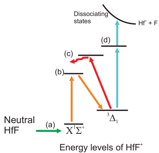
Figure 1.6: Major state manipulation steps that had to be performed to enable to eEDM measurement: state preparation of \text{HfF}^+ in a single desired quantum level using (a) photoionization and (b) Raman transfer, and state detection using either (c) laser-induced fluorescence or (d) photodissociation. This figure has been adapted from [81, 16].
