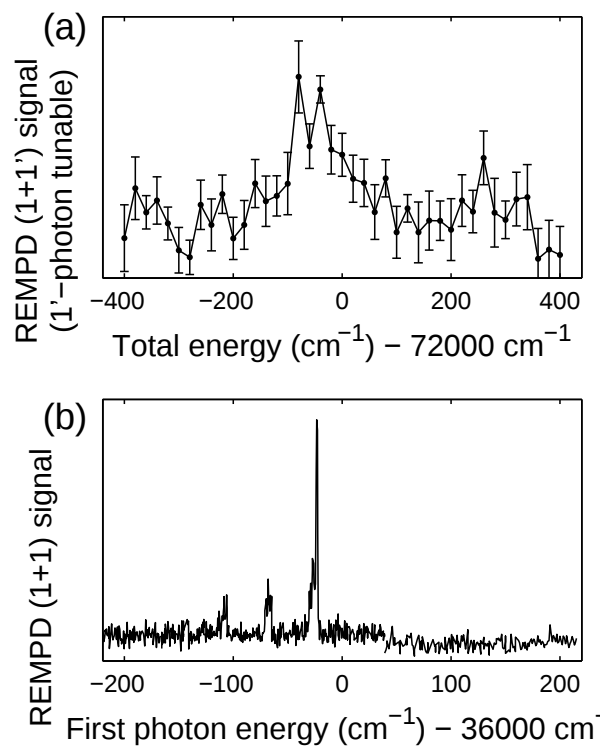
Figure 6.8: (a) Dissociation resonance accessed by two photons of total energy 71600–72400 \text{cm}^{-1} , recorded by tuning the first photon to 35976 \text{cm}^{-1} and scanning the frequency of the second photon. When scanning the dissociation resonance in (a), care was taken to step cleanly over any one-photon transitions shown in (b). (b) \text{HfF}^+ transitions accessed by a single photon of energy 35800–36200 \text{cm}^{-1} .
