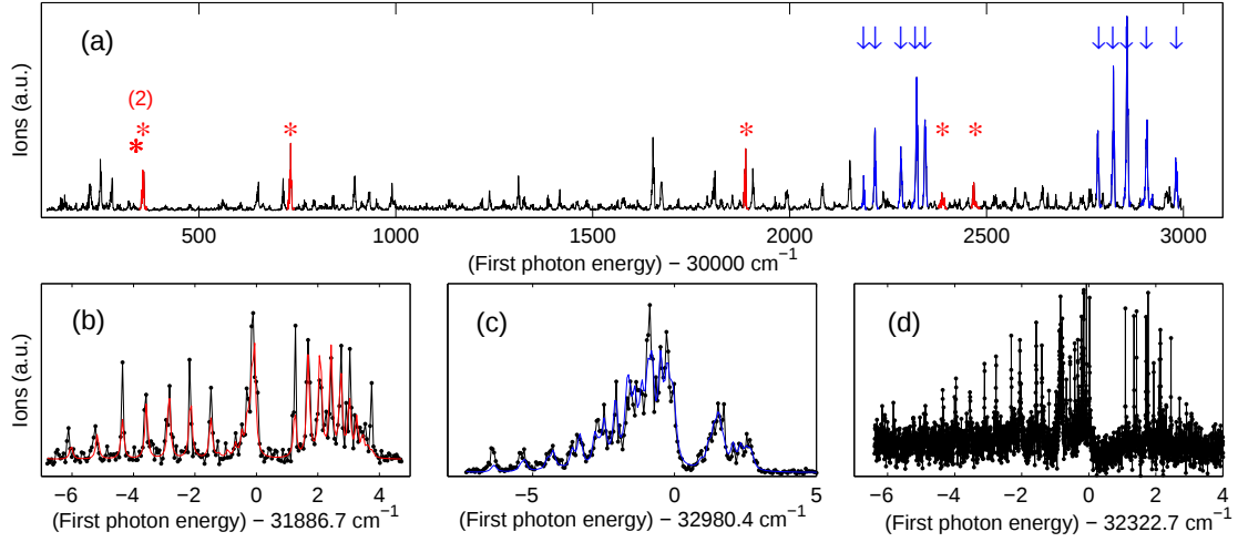
Figure 2.3: (a) Coarse (1+1) REMPI scan of excited HfF states near 30000 cm -1 . The ion signal shown is the integrated ion signal for all five HfF isotopologues. Two main types of transitions have been identified in this survey scan: \Omega' = 3/2 \leftarrow \Omega'' = 3/2 (marked by asterisks, typical spectrum shown in (b)) and \Pi_{1/2} \leftarrow \Omega'' = 3/2 (marked by arrows, typical spectrum shown in (c)). (b) Detailed (1+1) REMPI scan of the {31.89} vibronic band. The red smooth curve is a contour fit to the data shown as connected black dots. (c) Detailed (1+1) REMPI scan of the {32.98} vibronic band. The blue smooth curve is a contour fit to the data shown as connected black dots. (d) High resolution (1+1') REMPI spectrum of the {32.32} vibronic band. Individual upper state rotational levels of opposite parity can be resolved.
