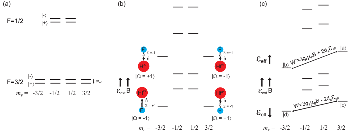
Figure 1.5: \text{HfF}^+ energy levels within the ^3\Delta_1, \nu = 0, J = 1 state. This figure is adapted from [45], with the energy ordering of the hyperfine levels switched to reflect the results experimentally obtained in this thesis. (a) In the absence of an external electric field, each hyperfine level possesses two closely-spaced states of opposite parity \{|+\rangle, |-\rangle\} , while the hyperfine m_F projections are degenerate. (b) With an external electric field (that also sets the quantization axis), the states of opposite parity are mixed and the hyperfine levels are split into (2F+1)/2 Stark manifolds, where the molecule internuclear axis \hat{n} is aligned parallel (anti-parallel) to the external electric field for the lower (upper) Stark manifold. (c) In the presence of a magnetic field parallel to \mathcal{E}_{\text{ext}} , the m_F sublevels undergo a Zeeman shift. The eEDM-sensitive transitions are denoted by \omega_{\text{eEDM}} , with the eEDM having oppositely signed contributions to \omega^u and \omega^\ell (see text).
