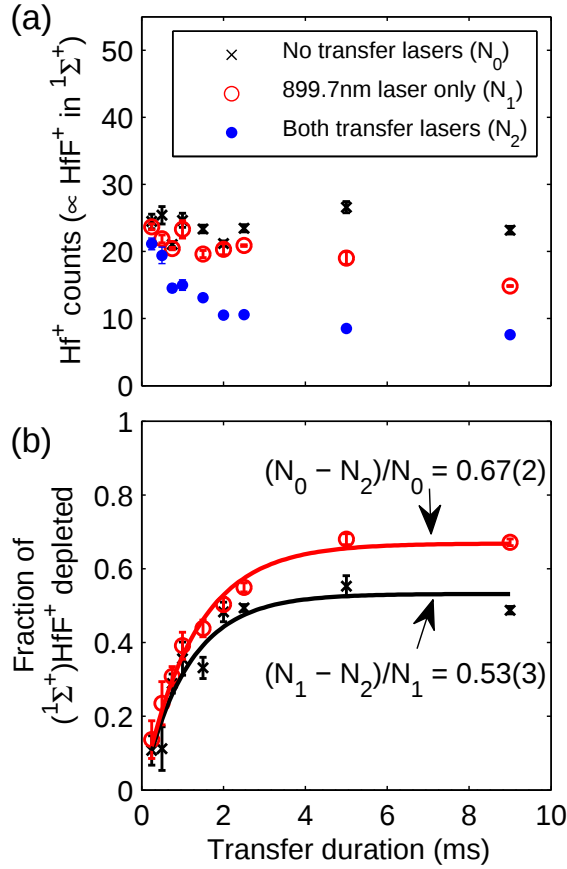
Figure 7.6: (a) HfF + ions (detected as dissociated Hf + ) as a function of transfer laser duration for the cases of (blue dots) both transfer lasers present, (red open circles) 899.7 nm laser present only, and (black crosses) no transfer lasers. The 899.7 nm laser causes a slow off-resonant optical pumping of HfF + out of the 1 Σ + state over time. The presence of both transfer lasers depletes the 1 Σ + ions more quickly. (b) Fraction of HfF + ions depleted from the 1 Σ + state, determined from the data shown in (a) as either (red) (N_1 - N_2)/N_1 or (black) (N_0 - N_2)/N_0 . The depletion fraction, which is expected to be the same as the transfer fraction, saturates after a few milliseconds of transfer time.
