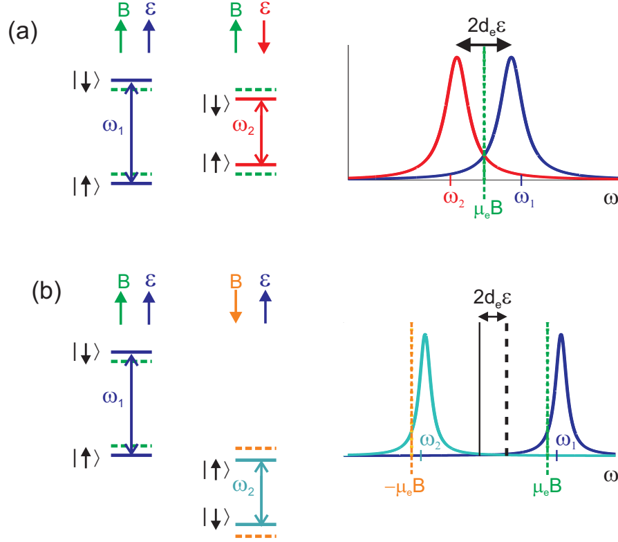
Figure 1.3: (The eEDM may be determined by measuring the electron spin-flip transition frequency in the presence of an external electric and magnetic field aligned parallel to each other, and then (a) reversing the direction of the electric field and taking the difference of the two transition frequencies, or (b) reversing the direction of the magnetic field and summing the two transition frequencies.
