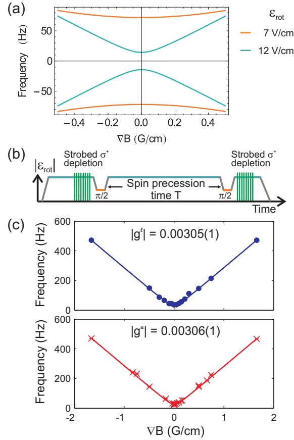
Figure 8.4: (a) Theory curves for the avoided crossing as a function of the rotating magnetic field (mocked up using \nabla B ), plotted for two different values of \epsilon_{rot} . (b) Ramsey sequence performed to measure the magnetic g-factor. The \pi/2 -pulses are ramps in \epsilon_{rot} , which can change the eigenstate at some finite magnetic field from, say, \approx |a\rangle to \approx (|a\rangle - |b\rangle)/\sqrt{2} . (c) The avoided crossing is experimentally mapped out for both the lower (blue dots) and upper (red crosses) Stark manifolds. The slopes of the avoided crossing give |g_F^\ell| = 0.00305(1) and |g_F^u| = 0.00306(1) .
