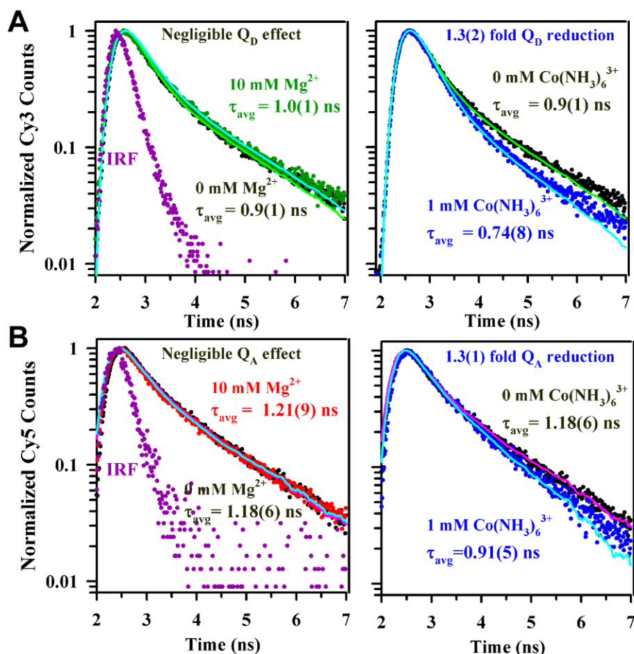
Figure 6.10 Fluorescence lifetimes of donor Cy3 (A) and acceptor Cy5 (B) as function of [cation]. 10 mM \text{Mg}^{2+} has no effect on the fluorescence lifetimes (left). Cobalt hexamine quenches the donor and acceptor to same extent. Lifetimes are fit to bi-exponential decays convoluted with the instrument response function (IRF shown in the left panel). The population-weighted average ( \tau_{\text{avg}} ) of the two lifetime components is shown. Uncertainties are indicated in parentheses. The effect of the added cation on the donor ( Q_D ) and acceptor ( Q_A ) is shown at the top of each graph (see supporting text).
