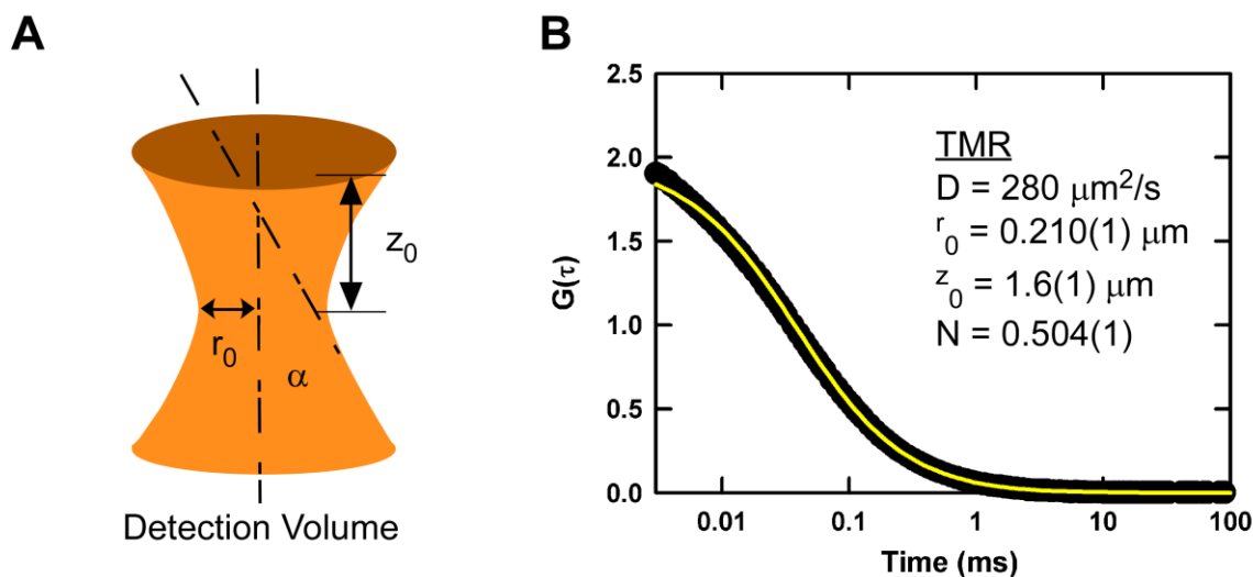
Figure 2.4 (A) Gaussian profile of the confocal detection volume with 1/e^2 radius intensity drop off in the lateral ( r_0 ) and axial ( z_0 ) dimensions. (B) Cross correlation of donor channels for tetramethylrhodamine (TMR) with a known diffusion coefficient ( D ) and fit to Eq. 2.7 to yield the r_0 , z_0 , and N (the mean occupancy of focus).
