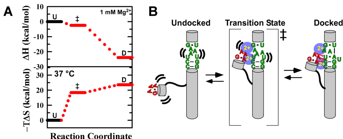
Figure 5.5 Proposed schematic mechanism for Mg 2+ -facilitated TL-R folding. (A) The entropic and enthalpic reaction coordinate for TL-R docking, where U, ‡, and D indicate the undocked, transition, and docked states. (B) The transition state is early and “compact”, i.e., requiring entropically disfavored proximity of the tetraloop and receptor and localization of counterions (e.g., Mg 2+ , blue circles), yet hydrogen bonding and base-stacking interactions in the docked state (red lines) are largely unformed. Docking increases the charge density of the RNA, permitting further Mg 2+ localization.
