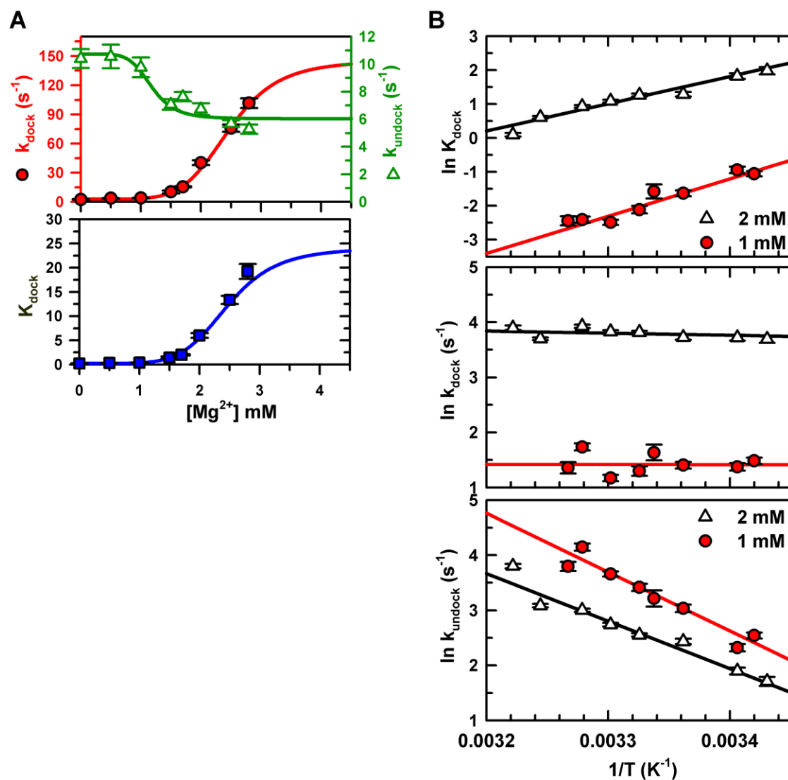
Figure 5.11 [Mg^{2+}] and temperature dependence of the tetraloop-receptor docking/undocking ( U_7 construct, Figure 5.1 A) at low [NaCl] (25 mM). (A) [Mg^{2+}] for k_{dock} , k_{undock} and K_{dock} fit to the four-state kinetic scheme as in Figure 5.2, yielding n = 6 \pm 1 , k_1 = 2.9 \pm 0.3 s^{-1} , k_2 = 145 \pm 50 s^{-1} , k_{-1} = 11 \pm 1 s^{-1} , k_{-2} = 6.0 \pm 0.3 s^{-1} , K_{Mg} = 2.5 \pm 0.3 mM , and K'_{Mg} = 1.2 \pm 0.2 mM . At low [Na^+] the Mg^{2+} cooperativity ( n ) is substantially greater than at 100 mM NaCl (Figure 5.2). (B) van't Hoff and Arrhenius plots yield the enthalpies and entropies of tetraloop-receptor docking/undocking at low [NaCl] , as summarized in Table 5-1 and Table 5-2.
