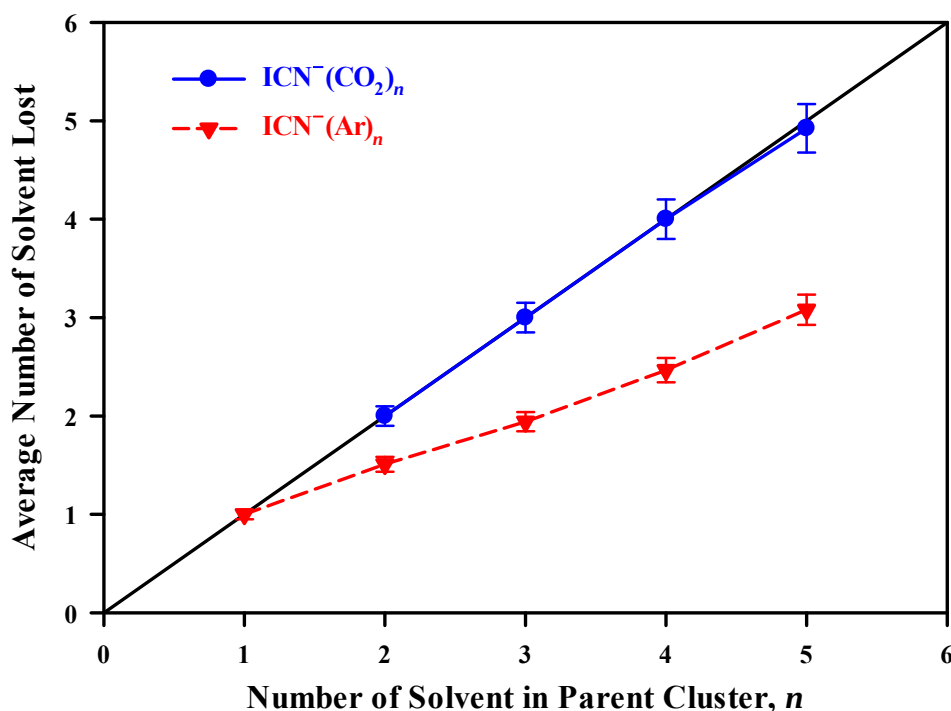
Figure 4.15 The average number of solvent lost from \text{I}^- -based and \text{ICN}^- -based photoproducts as a function of parent cluster size, n , following 500 nm excitation of \text{ICN}^-(\text{CO}_2)_n and \text{ICN}^-(\text{Ar})_n . See Chapter III for \text{ICN}^-(\text{Ar})_n photofragmentation results. The solid black line corresponds to the evaporation of all solvent from the parent cluster and is shown as a guide. The error bars correspond to a 5% standard deviation.
