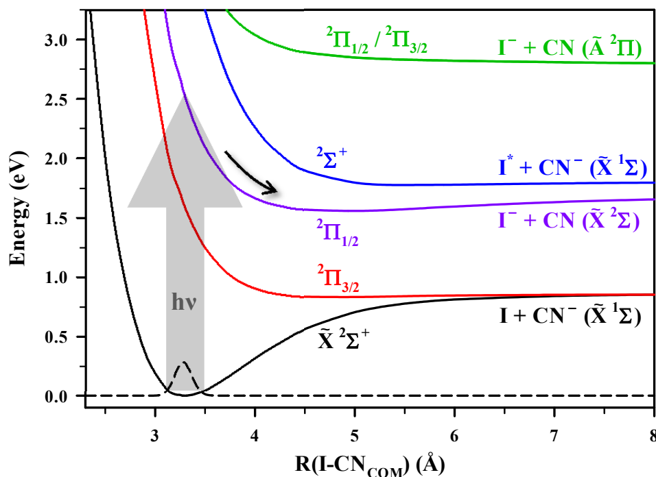
Figure 3.1 Schematic potential energy curves (based on Ref. 66) for the \text{ICN}^- ( \tilde{X}^2\Sigma^+ in black and ^2\Pi_{1/2} in purple) as a function of the I–CN center of mass distance. The black dashed line shows the probability amplitude of the ground-state wave function for \text{ICN}^- . The black arrow illustrates photoexcitation and subsequent dissociation (3.1).
