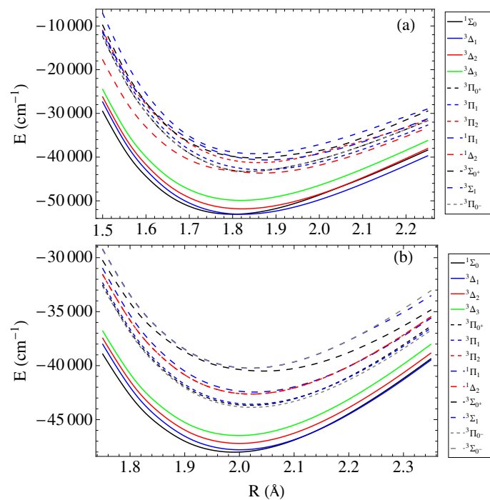
Figure 3.8: Results of the many state calculation on \text{HfF}^+ (a) and \text{ThF}^+ (b) at the RHF-MCSCF+MRCI+SO level of theory.
