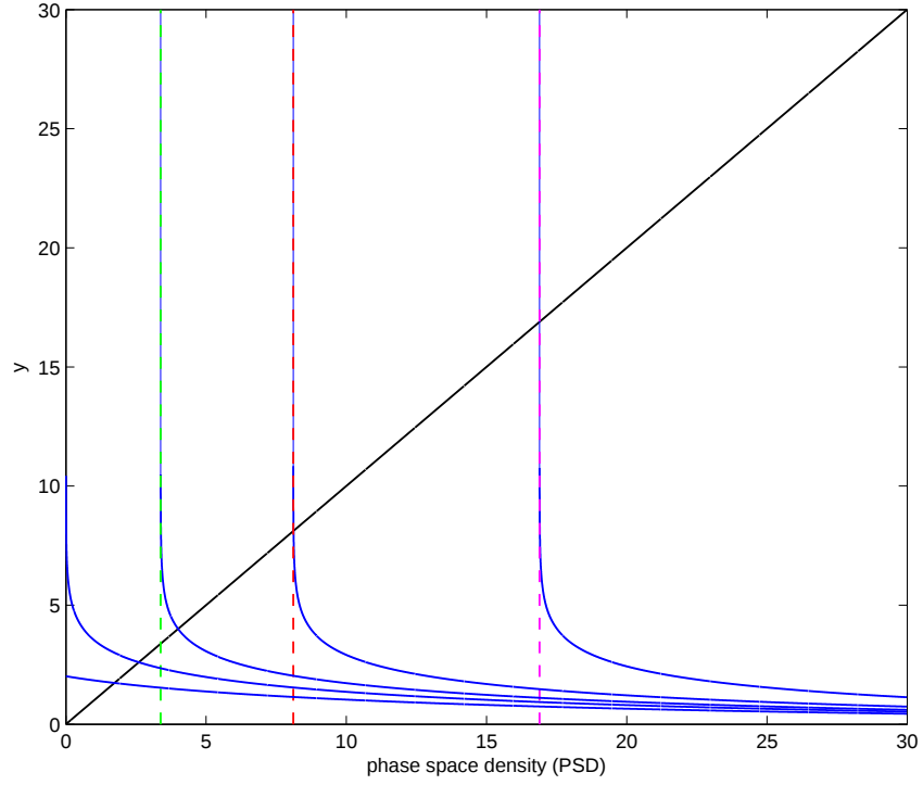
Figure 4.1: The solution of Eq. (4.4) for five different chemical potentials. The blue curves represent y = -\ln(1 - e^{-(\theta_j(\vec{r}) - \mu_j(\vec{r}))/k_bT}) for five different chemical potentials \mu'/k_bT , -0.14, 0, 0.1, 0.24, and 0.5 (from left to right). The black curve represents y = n\lambda_{db}^2 . The intersection for each blue curve and the black curve gives the density that satisfies Eq. (4.4). The three dashed lines indicate the values of the phase-space density where the last three blue curves diverge.
