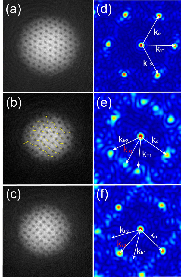
Figure A.3: Images of rotating condensates pinned to an optical lattice at \Omega_{OL} = \Omega_c = 0.866\omega_r with pinning strength U_{pin}/\mu =(a) 0.049 (b) 0.084 (c) 0.143, showing the structural cross-over of the vortex lattice. (a)–(c) are the absorption images of the vortex lattices after expansion. (d)–(f) are the Fourier transforms of the images in (a)–(c). k_o is taken by convention to be the strongest peak; k_{tr1} , k_{sq} , and k_{tr2} are at 60^\circ , 90^\circ , and 120^\circ , respectively, from k_o .
