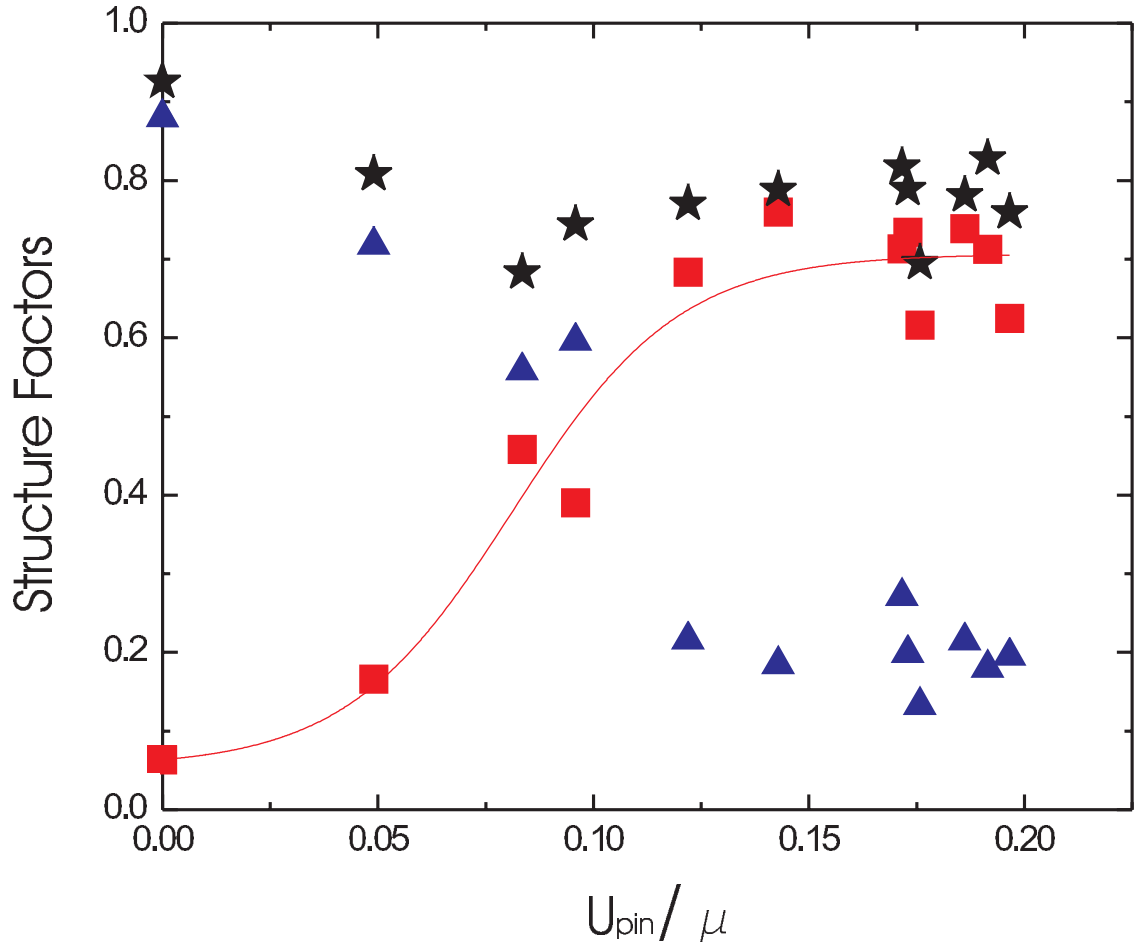
Figure A.4: Structure factors (a) |S(k_{sq})| (■), (b) |S(k_{tr})| (▲) (average of |S(k_{tr1})| and |S(k_{tr2})| ), and (c) |S(k_o)| (★) versus the strength of the pinning lattice at the commensurate rotation rate \Omega_c . |S(k_{sq})| is fitted by [75]. The fitting leads to a maximum value 0.707 of |S(k_{sq})| . An ideal square vortex lattice would have |S(k_{sq})|=1 .
