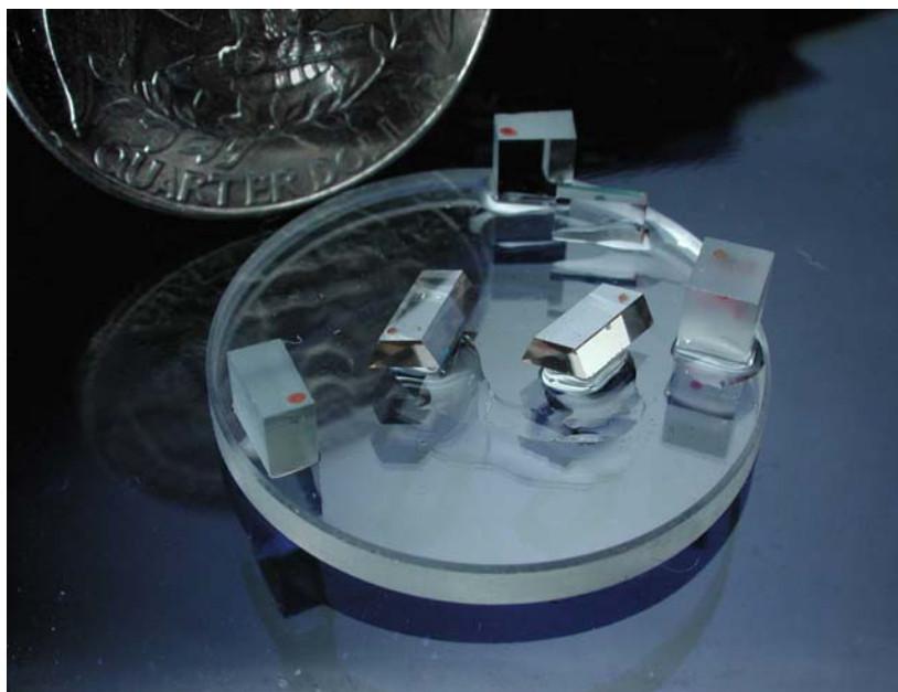
Figure 2.7. Photograph of the autotuning filter using free space miniature optics.
