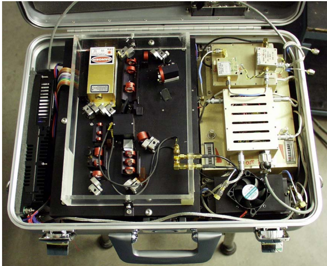
Figure 3.17: Photograph of the “suitcase project.” The two coaxial cables visible in the top right corner receive electrical signals directly from the patch antennas placed on the focal arc of the antenna array. The bigger gold-colored box contains the LNAs and the down converting electronics. The output is amplified by power amplifiers sitting under the visible cooling fan (there is another one under the
