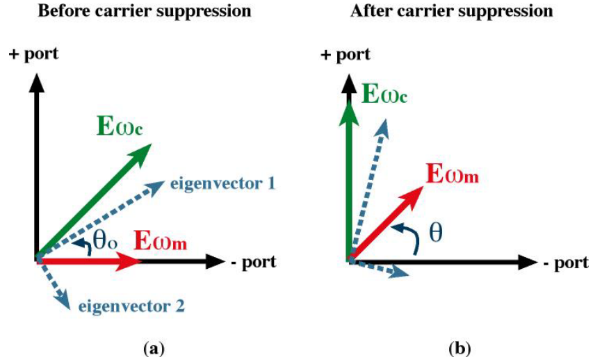
Figure 3.12. 2D representation of single mode two-beam coupling. (a) In the case of carrier suppression the input to the minus (“-”) port is a modulated laser beam while the input to the plus (“+”) port is a non-modulated beam from the same laser. (b) Nonlinear coupling between the beams causes the energy in the carrier at the minus port to be transferred to the plus port at the output.
