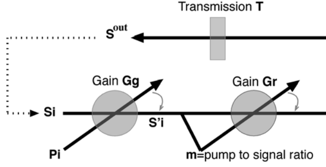
Figure 2.16: Illustration of the notations used in the equations of this section.
