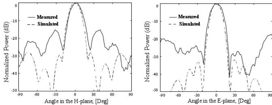
Figure 3.5 Measured (solid line) H-plane (on the left) and E-plane (on the right) radiation patterns at 9.9 GHz have higher sidelobes than the simulated patterns for a uniformly illuminated array (dashed line). This is due to the non-uniform amplitude and phase associated with the near-field spatial feed. The simulated patterns are calculated using the measured radiation pattern of the patch element
