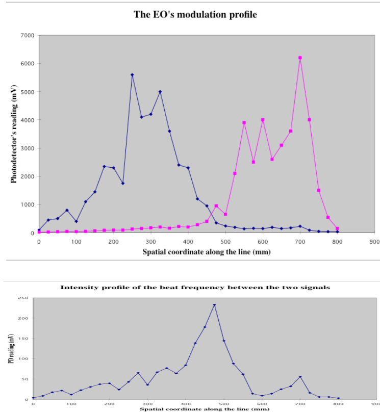
Figure 3.10. Modulation profile at the output of the two-channel electro-optic modulator along the optical beam.
