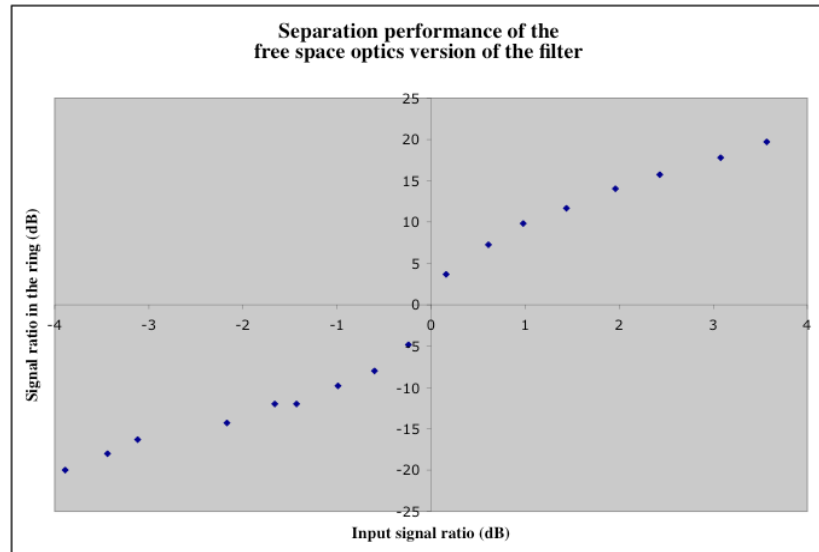
Figure 2.14: Separation curve taken with the filter shown in Figure 2.7
