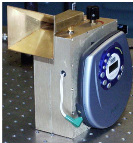
Figure 3.2. Photograph of the battery operated transmitters. The CD player provides the audio signal that modulates the transmitted microwaves.
