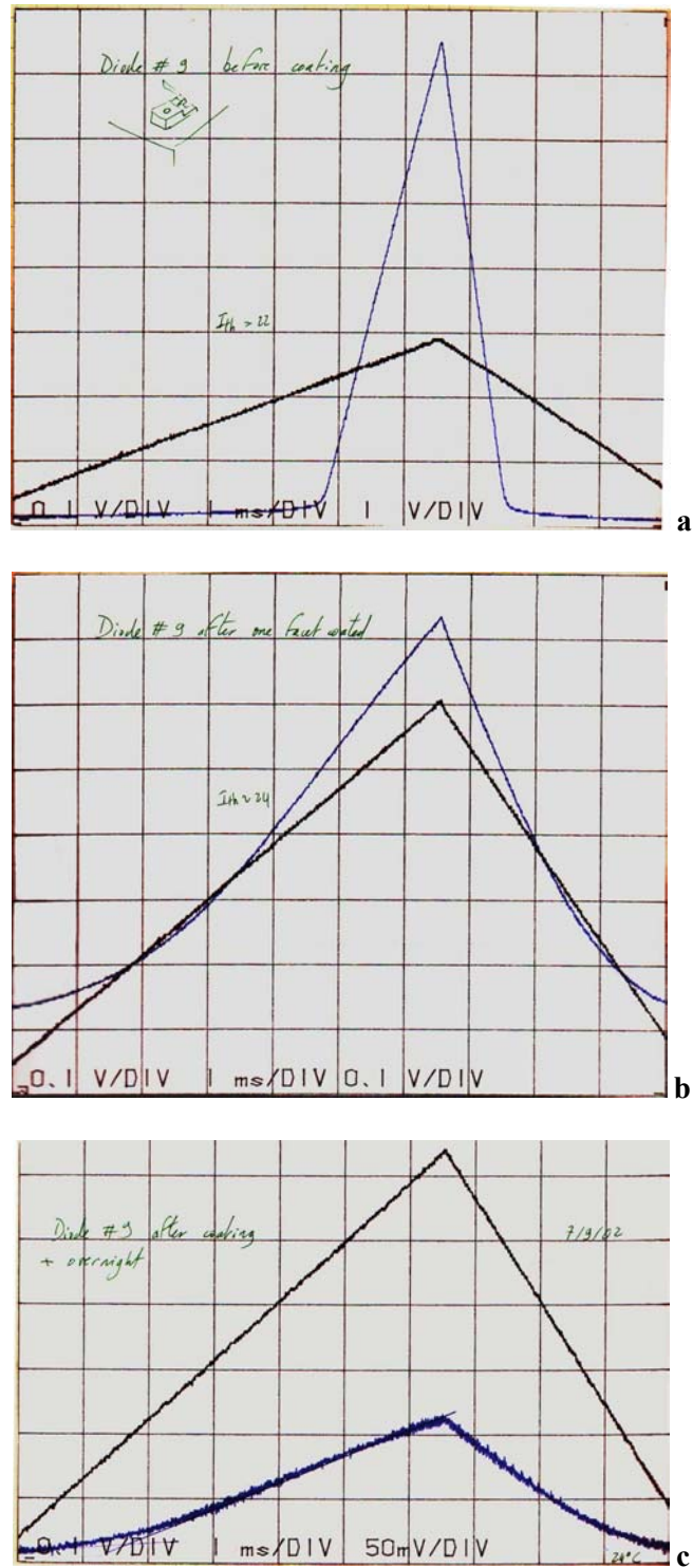
Figure 4.2. PI curves of a laser diode. The triangular black curves represent the current passing through the diode.
