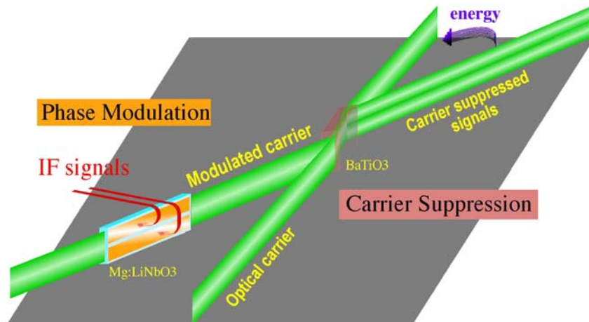
Figure 3.11. Two-beam coupling in a photorefractive barium titanate crystal ( \text{BaTiO}_3 ) suppresses the optical carrier.
