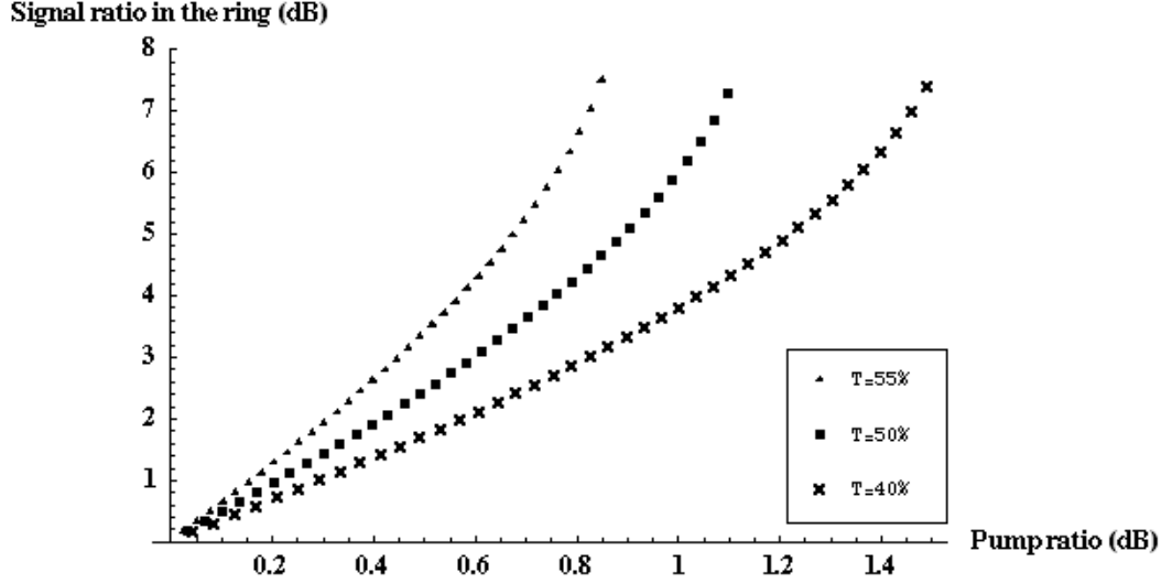
Figure 2.20. S_1/S_2 vs. P_1/P_2 curve for T=0.55 , 0.50 , and 0.40 left to right ( Gg=Gr=10 , m=25 ).
