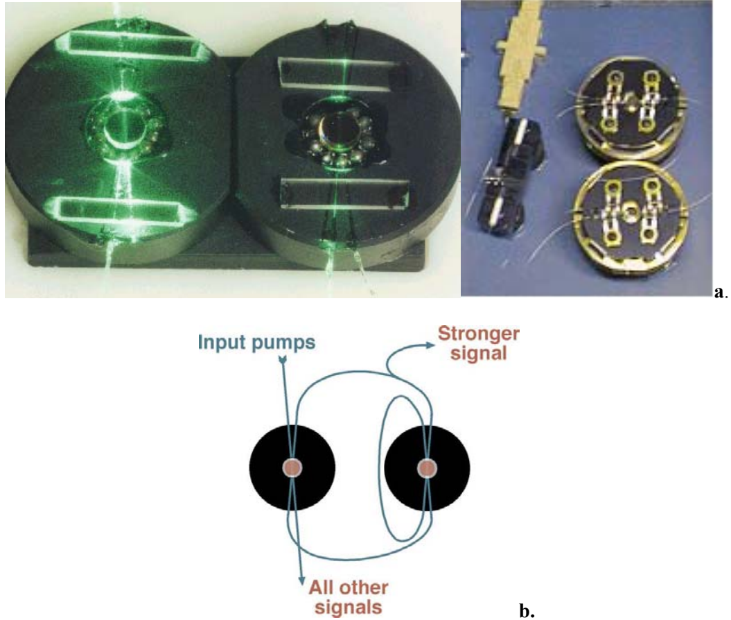
Figure 2.6. a) Photographs of the two fiberized autotuning filter versions. The crystals are slabs of spheres as it wastes less material than whole spheres. b) Design of the autotuning filter using fibers and spherical crystals.
