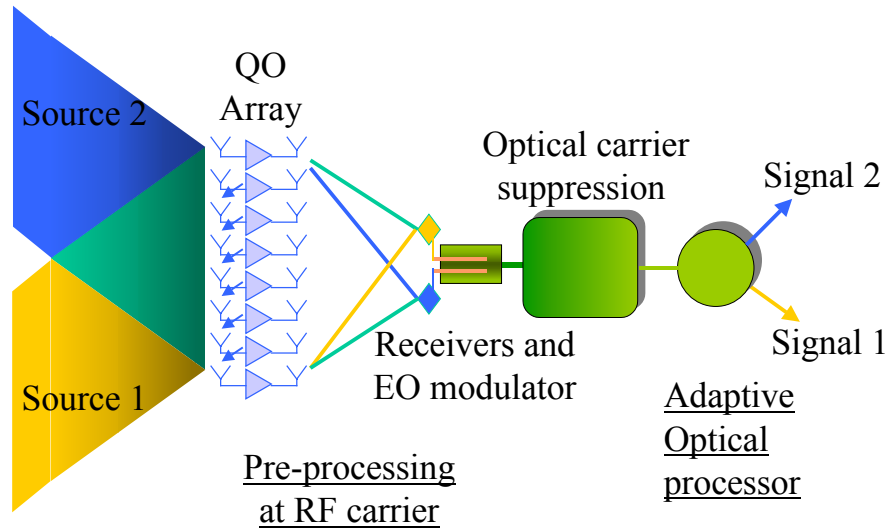
Figure 3.1: Diagram of the prototype optically smart antenna array.
