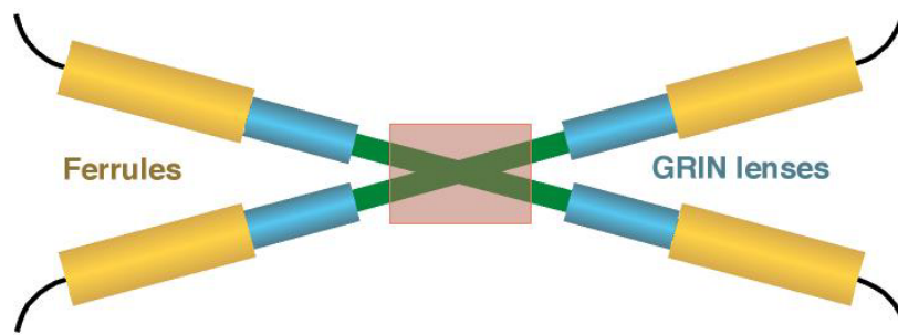
Figure 2.4. GRIN lenses collimate (and refocus) the light coming out of (or into) a fiber held by a ferrule.
