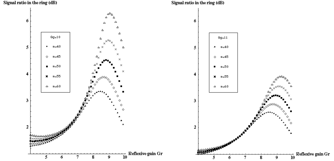
Figure 2.21. Left side: S_1/S_2 vs. Gr for m=60, 55, 50, 45 , and 40 from top to bottom with T=0.5 , Gg=10 , and P_1/P_2=0.2 dB. Right side: same values except Gg=11 .
