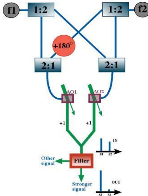
Figure 2.12: AO test bed with mixtures of two signals driving each AO. Each signal is split in two and recombined with half of the other signal. A 180-degree phase shift is added to one half of S2 before it is recombined.
