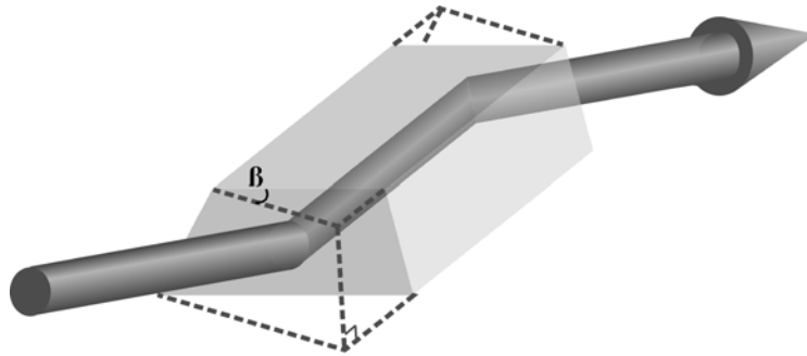
Figure 2.8. The "gold bar" shaped cut of photorefractive crystals suppresses unwanted oscillations arising between otherwise parallel faces.
