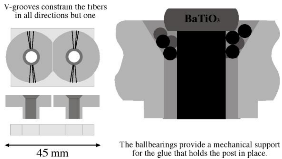
Figure 7.2 Mechanical mount for the first version of the autotuning filter with spherical photorefractive crystals (see Figure 2.6.a.)
