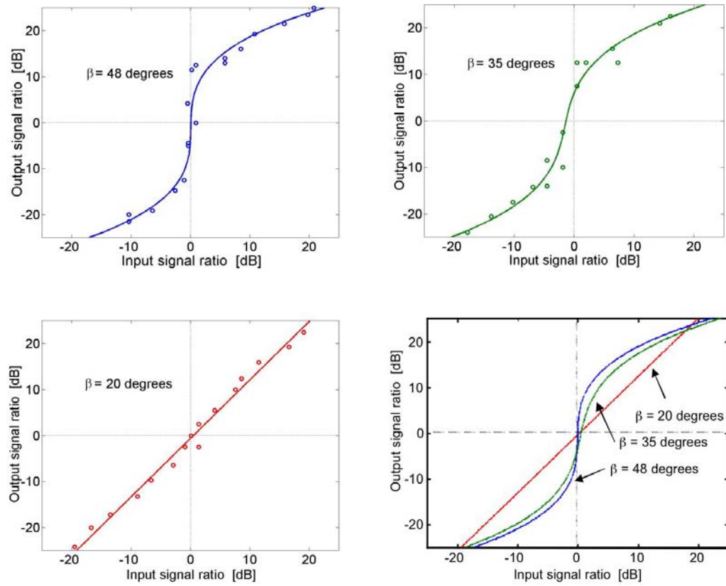
Figure 3.20. Signal extraction properties of the adaptive system parameterized by the mutual angle between the transmitters.
