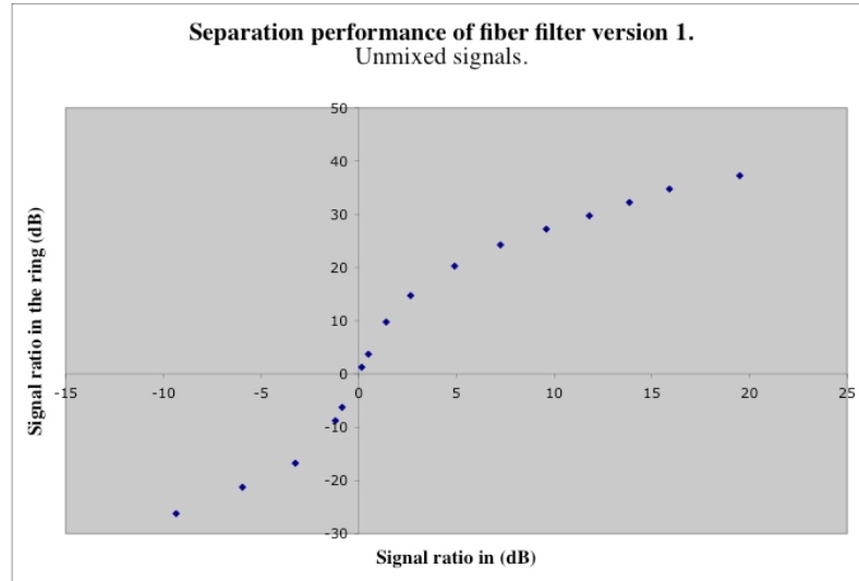
Figure 2.11. Separation curve taken with the filter on the top left-hand side of Figure 2.6
