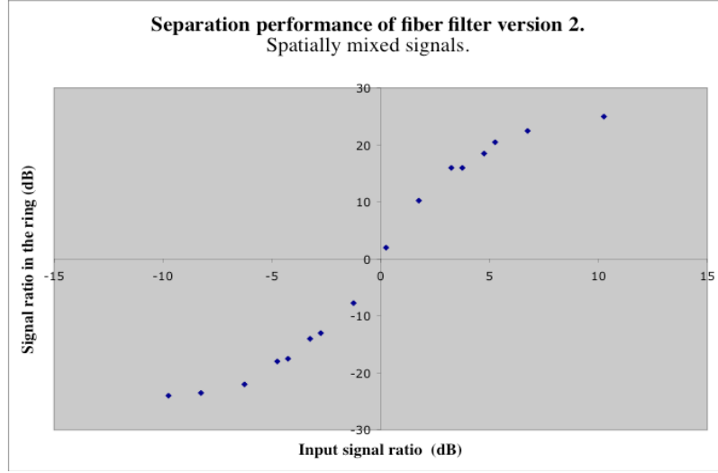
Figure 2.13: Separation curve taken with the filter shown on the top right-hand side of Figure 2.6 and with the test bed of Figure 2.12
