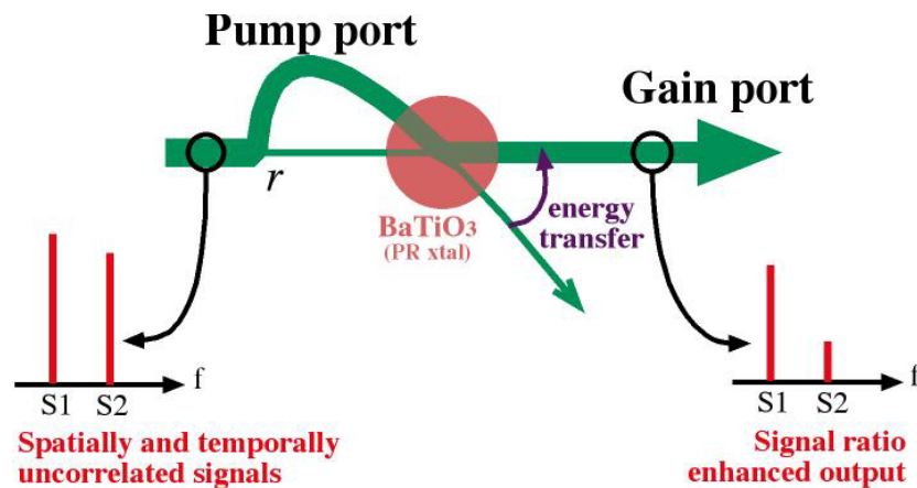
Figure 2.3. Reflexive coupling is a photorefractive selective loss element. It induces loss inversely proportionally to the strengths of signals.
