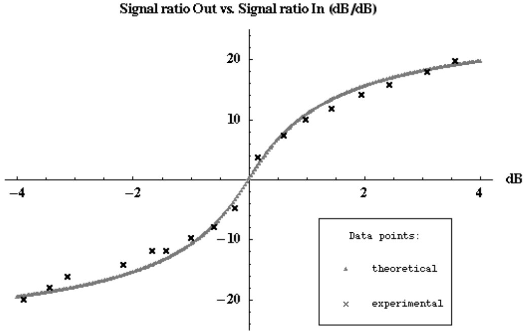
Figure 2.23. Separation performance of the filter. The smooth gray curve shows calculated data points using the first principal component extraction model. The slope at the origin is 15 dB/dB. This is in contrast to the experimental data points (in black) which show a slope at the origin of 26dB/dB.
