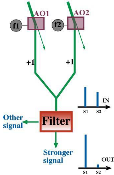
Figure 2.10. Schematic of the AO test bed used to evaluate the separation performance of the autotuning filters.
