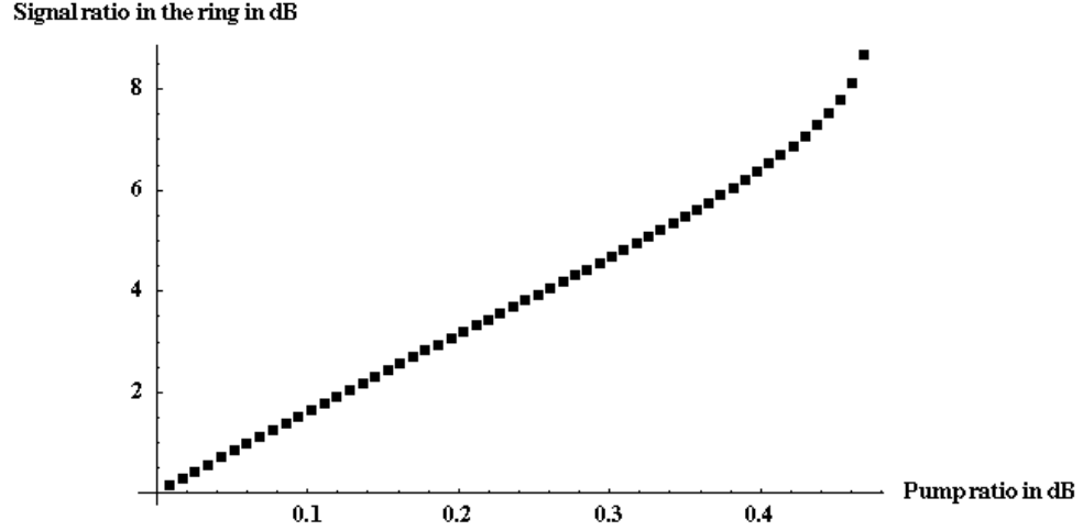
Figure 2.18. The Log-Log plot of the S_1/S_2 vs. P_1/P_2 curve shows a linear region when both signals are oscillating in the ring and a rapid increase toward infinity as the input signal ratio approaches the boundary value where the weaker signal disappears. The parameter values are Gr=Gg=10 , m=50 , and T=0.5 .
