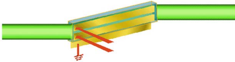
Figure 3.8. Electro-optic modulation: a channelized electro-optic modulator made from magnesium doped lithium niobate crystal ( \text{Mg:LiNbO}_3 ) imposes spatial and temporal modulation on the optical carrier.
