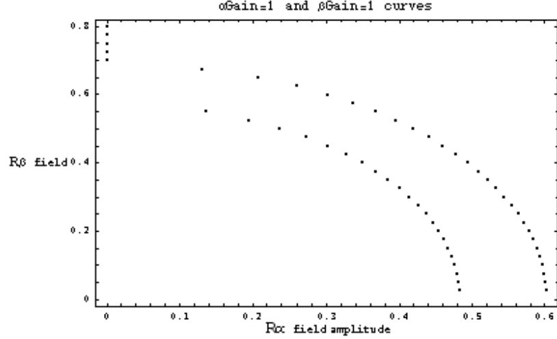
Figure 2.25. Gain curves for two spatially and temporally orthogonal signals.
