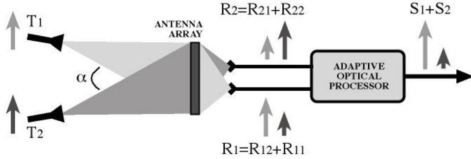
Figure 3.19. Diagram defining the context of the end-to-end system measurements.
