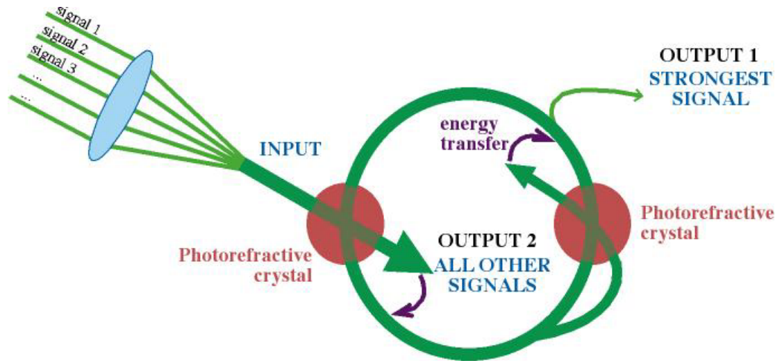
Figure 2.2. Schematic of the autotuning filter's design. The two-beam coupling occurring in the crystal on the left of the figure provides gain to the ring. The two-beam coupling taking place in the crystal on the right imposes loss on the ring signals inversely proportionally to their relative intensities.
