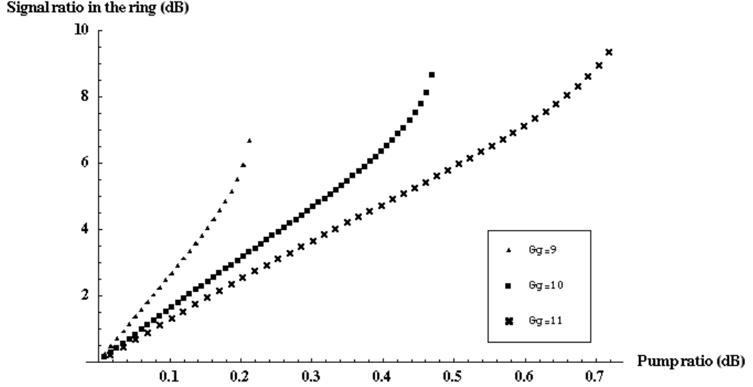
Figure 2.19. S_1/S_2 vs. P_1/P_2 curve for Gg=9 , 10, and 11, left to right ( T=0.5 , Gr=10 , m=50 ).
