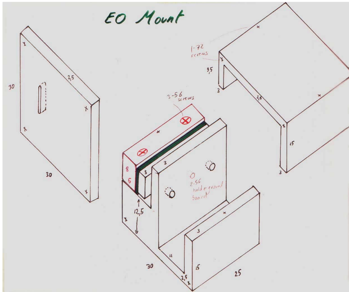
Figure 7.4. EO mount that holds the 0.3x7x30 mm crystal pressed against a piece of foam.
