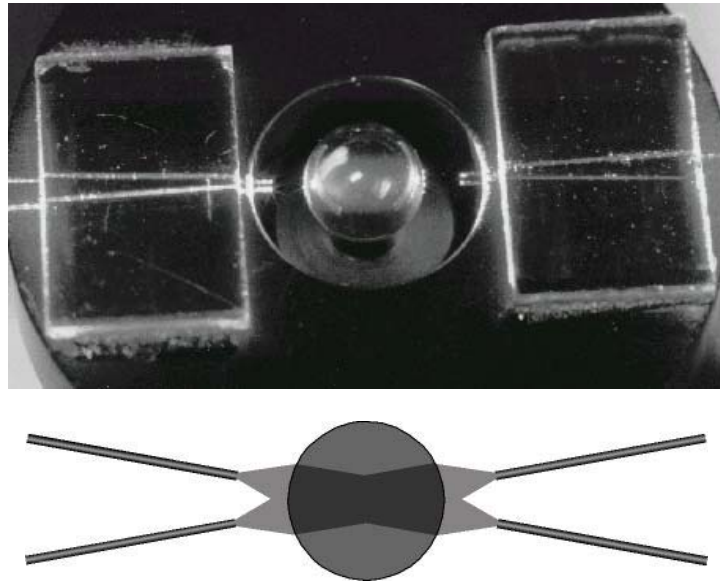
Figure 2.5. \text{BaTiO}_3 spherical crystals double as lenses to couple light from two fibers into two other fibers.
