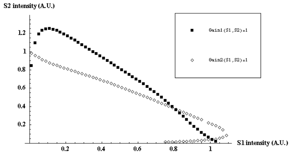
Figure 2.17. The intersection of two curves represent the pairs of (S_1, S_2) that yield G_1=G_2=1 .
