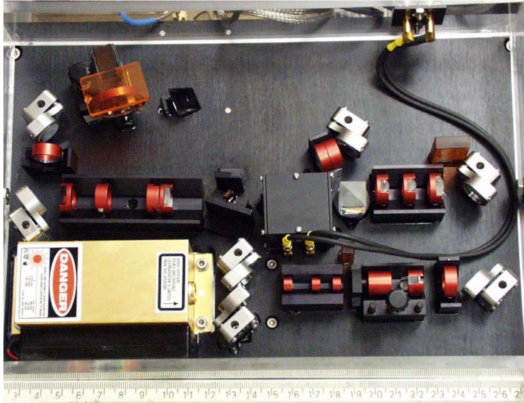
Figure 3.16: Photograph of the 8x11 inch optical stage.
