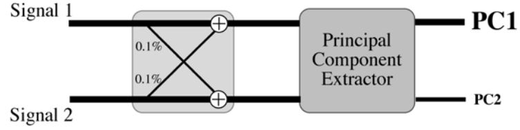
Figure 2.22. Simple model of our filter as a principal component extractor. The mixing on the left hand-side accounts for the spatially finite size of the photorefractive gratings that allows one pump beam to weakly diffract off of the other pump's grating.
