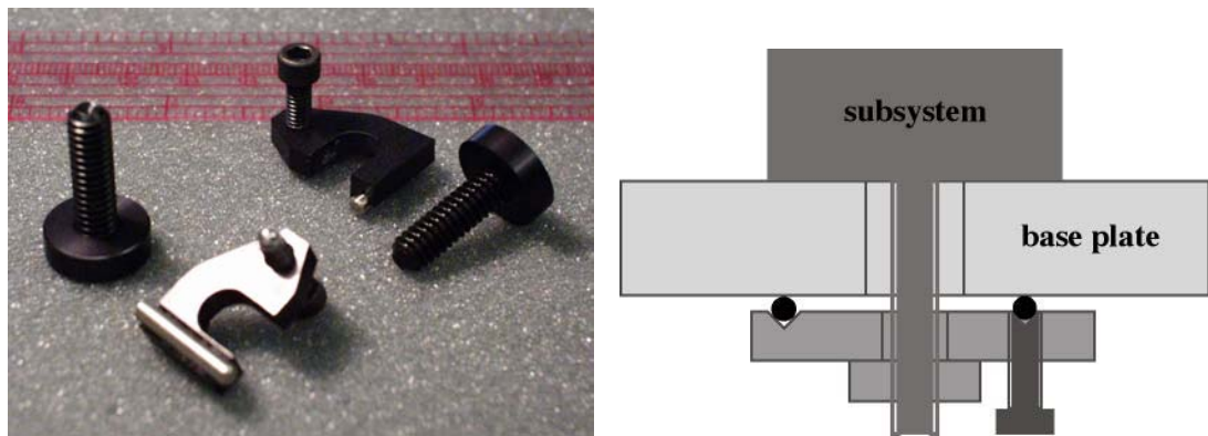
Figure 3.15: Photograph and picture of the inverted table clamps. A 1/4-20 screw with a threaded ring attach to every subsystem on the base plate. A u-shaped piece with an integrated screw pulls down on the ring thus immobilizing the sub sytem on the base plate.
