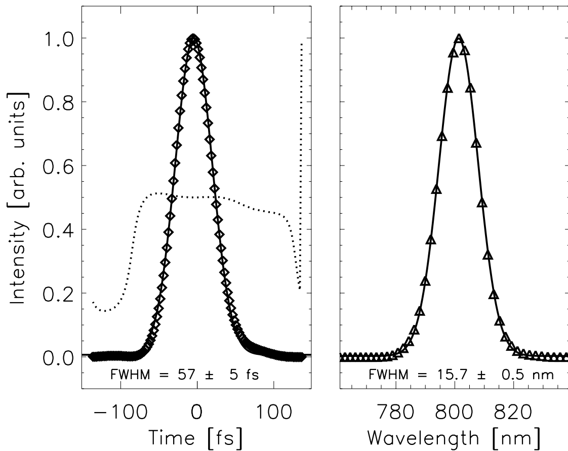
Figure 2.3: The temporal (left) and spectral (right) profile of the seed pulse from the Tsunami Ti:Sapphire laser measured with a commercial FROG instrument available in the JILA Keck labs. The dotted line is a measurement of the phase of the electric field across the pulse, or the amount of frequency chirp in the pulse. A flat phase indicates no frequency chirp across the pulse.
