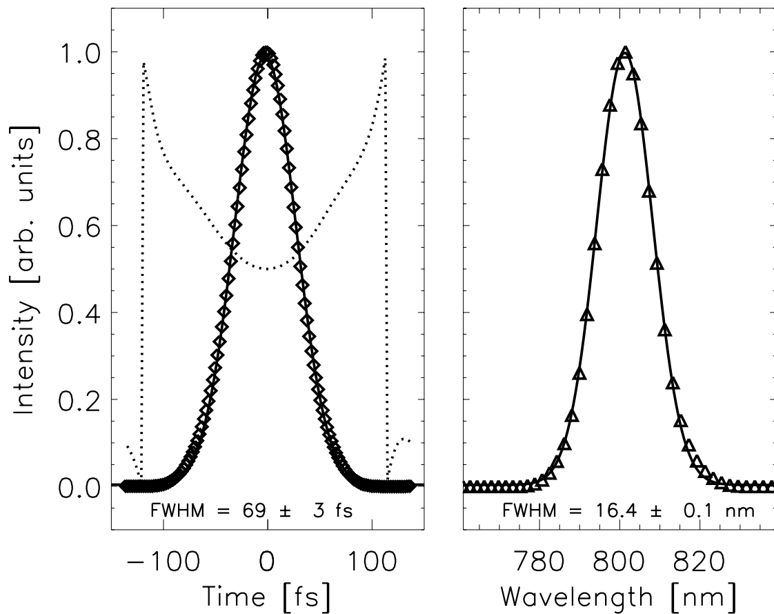
Figure 2.5: The temporal (left) and spectral (right) profile of the pulse from the amplified Ti:Sapphire laser measured with a commercial FROG instrument available in the JILA Keck labs. The slight curvature in the dotted line (representing the phase of the electric field) indicates a slight frequency chirp from the amplification process as compared to the seed pulse.
