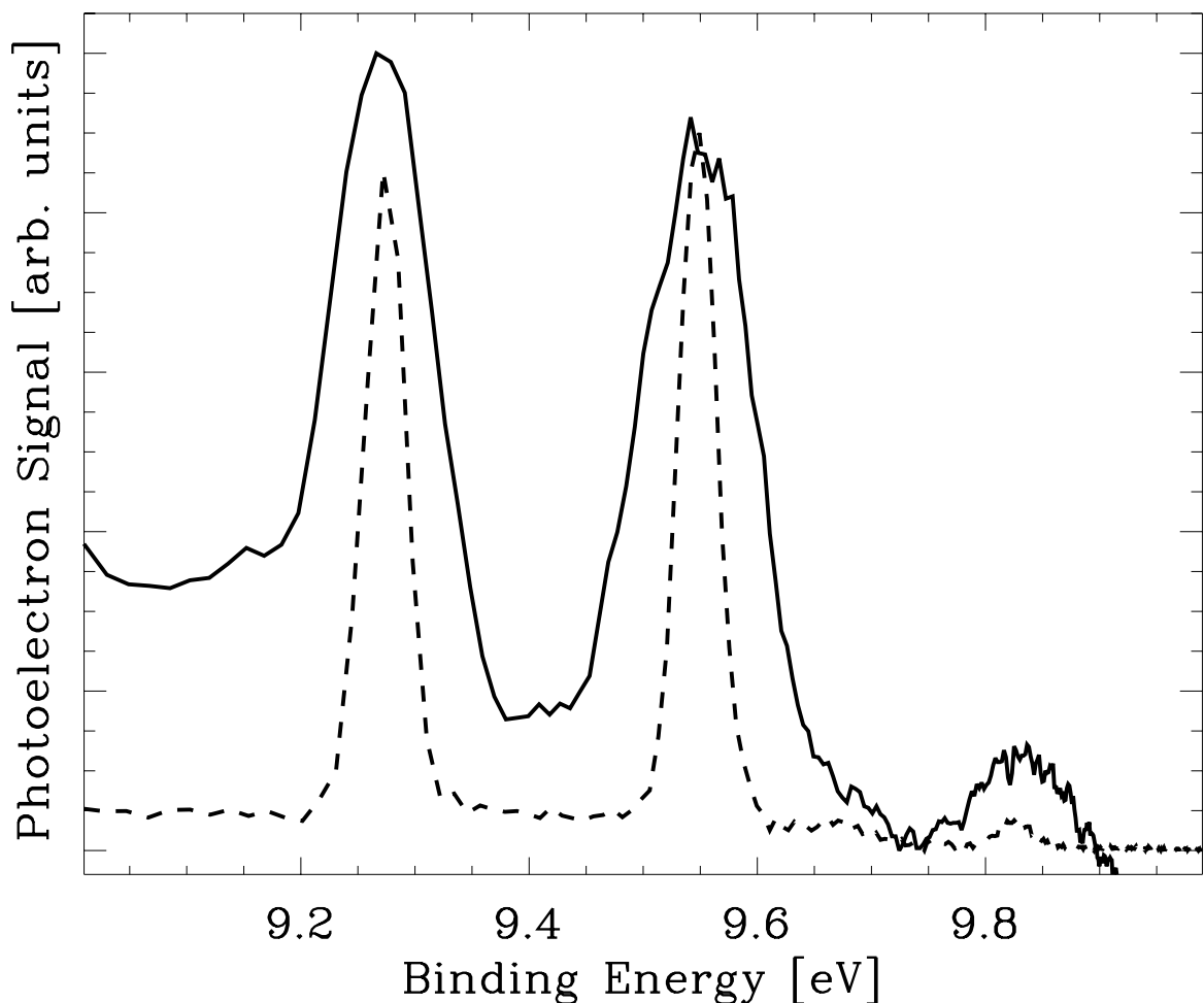
Figure 4.1: Photoelectron spectrum of NO gas taken with the 9th harmonic of a long pulse, narrowband Nd:YAG laser, E_{h\nu}=10.496 eV (dashed line). Here the inherent resolution of the magnetic bottle spectrometer is seen in the peak widths. The vibrational progression of the \text{NO}^+ ground state gives rise to the three peaks separated by \approx 0.28 eV. The solid line shows the same vibrational progression, but acquired with the 7th harmonic (centered at E_{h\nu}=10.91 eV) of the fs Ti:Sapphire laser. The broadening of the peaks is due to the energy bandwidth of the 7th harmonic. The height discrepancy in the highest binding energy peak between the Nd:YAG laser and the 7th harmonic of the Ti:Sapphire laser is due to the efficiency of the photoelectron spectrometer at different photoelectron energies. Though these peaks have the same binding energy, the dashed line peak at 9.8 eV corresponds to very low photoelectron energy, where the collection efficiency is quite low.
