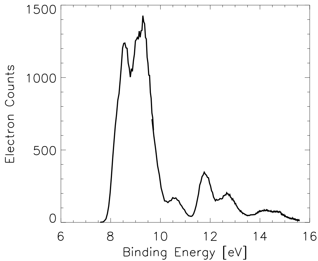
Figure 3.10: The photoelectron spectrum of \text{CH}_2\text{I}_2 with the 17th harmonic of 800 nm.
