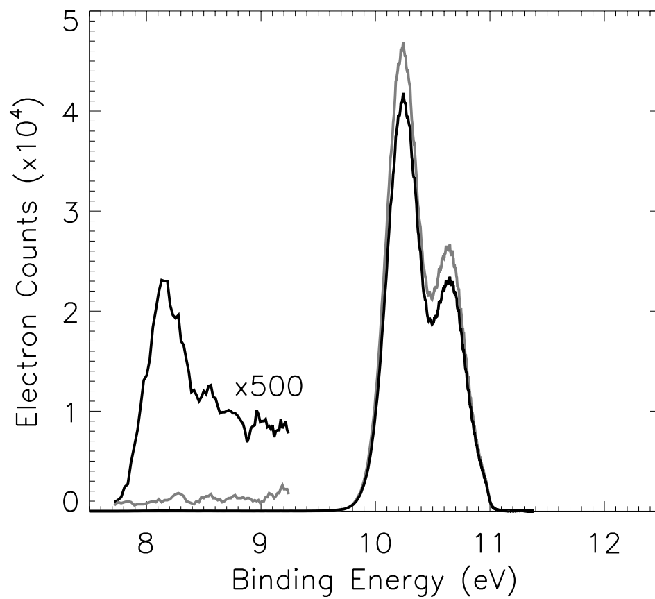
Figure 5.6: An expanded photoelectron spectrum of \text{Br}_2 with (black) and without (gray) the 527 nm excitation laser.
