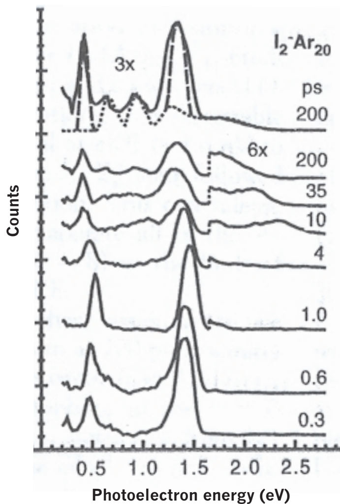
Figure 1.7: An example of a time-resolved photoelectron experiment from ref. [3]. The photoelectron spectrum of \text{I}_2^-(\text{Ar})_{20} clusters is shown at various time-delays between the pump and probe pulses.
