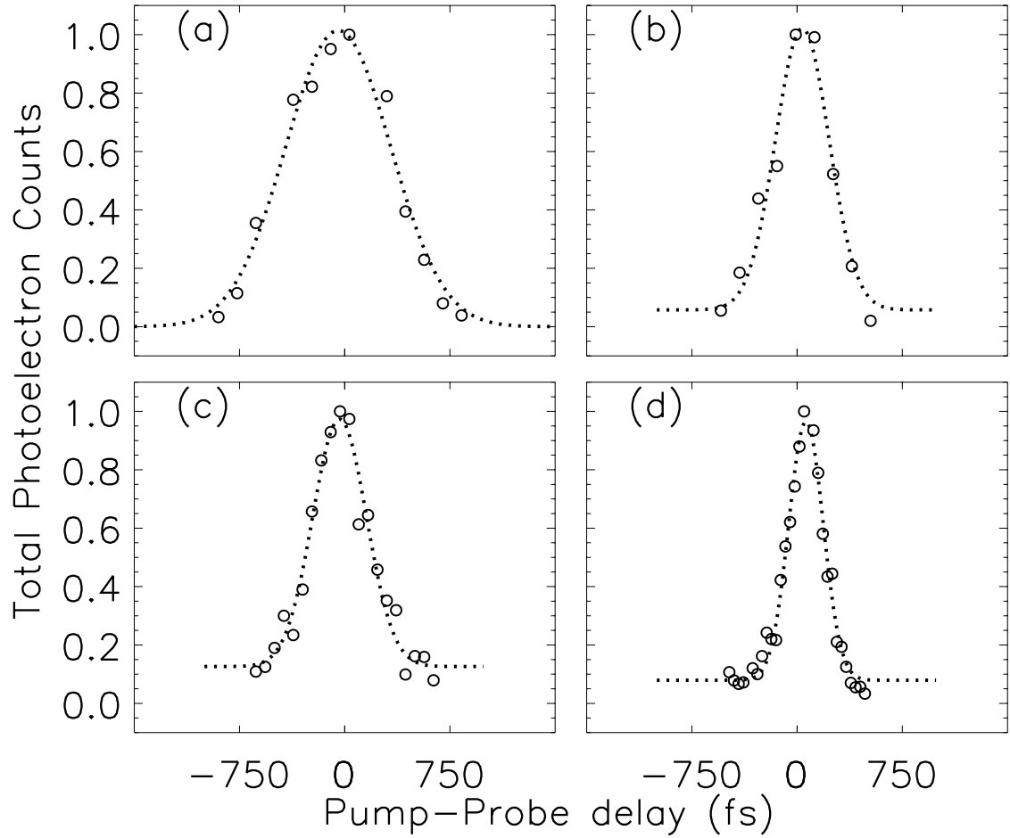
Figure 6.5: Cross-correlation traces of the 17th harmonic + 400 nm in Xe. (a) Toroidal grating rotated to 1st order diffraction, concave grating at 0th order reflection, iris open (8mm), FWHM = 882 \pm 105 fs; (b) as (a) except iris at 1 mm, FWHM = 449 \pm 64 fs; (c) Both toroidal and concave gratings rotated to 1st order diffraction, iris open (8mm), FWHM = 440 \pm 25 fs; (d) as (c) with iris at 1mm, FWHM = 288 \pm 12 fs.
