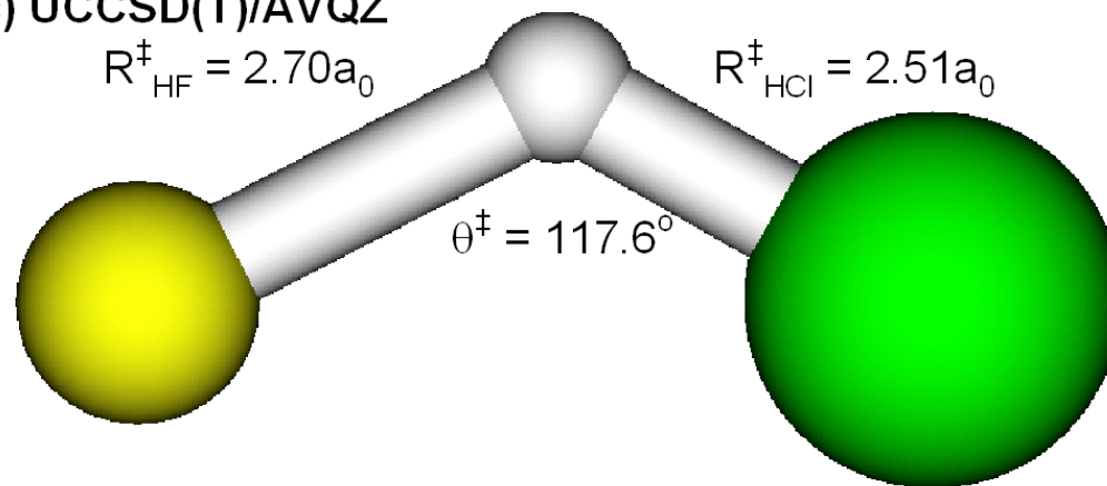
Figure 5.3: F-H-Cl transition state geometry at various levels of theory, all confirming a sharply bent transition state: (a) MRCI+Q/AVTZ; (b) MRCI+Q/CBS/Scaled; UCCSD(T)/AVQZ.
