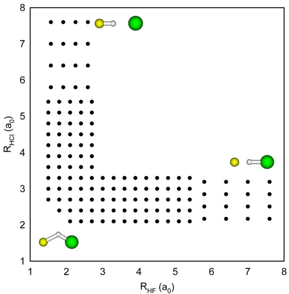
Figure 6.6: Grid of distributed Gaussian locations used to fit the \beta coupling surface.
