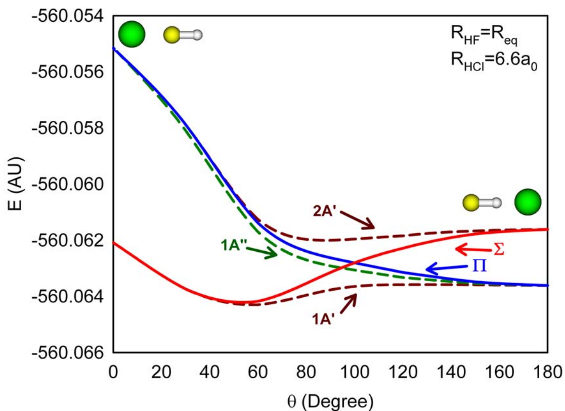
Figure 6.3: A 1D angular cut through full 3D adiabatic and diabatic surfaces in the exit channel, with R_{HF} = R_{eq} and R_{HCl} = 6.6 a_0 . The adiabats and diabats are asymptotically equal at collinear geometries, but strongly avoid as the symmetry is lowered from C_{\infty v} .
