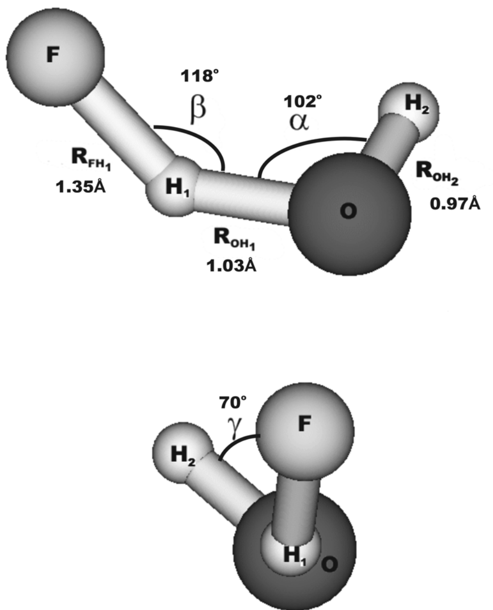
Figure 4.1: The internal coordinates used for specifying F + H_2O geometries. The geometry is given for the 5-state MCSCF transition state.
