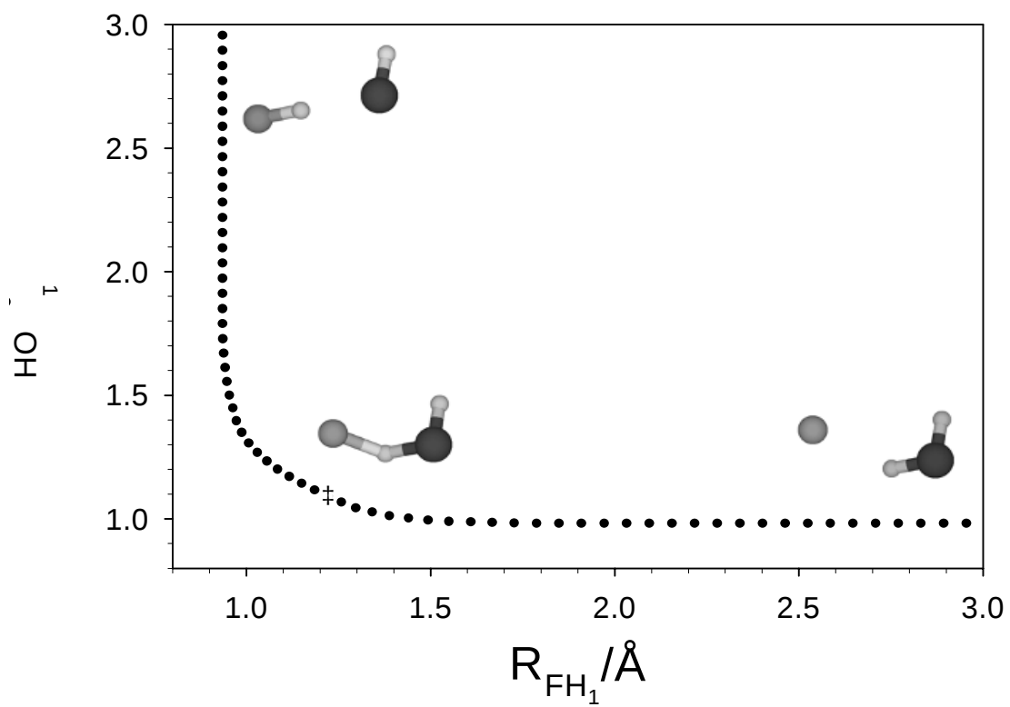
Figure 4.2: A 2D projection ( R_{\text{FH}_1} and R_{\text{OH}_1} bond distances) of the full 6D reaction path calculated at the 5-state MCSCF level. This 6D reaction path is used throughout the paper.
