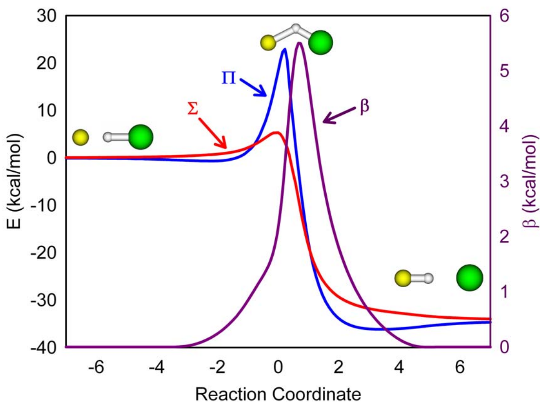
Figure 6.9: V_\Sigma and V_{\Pi x} diabats along the reaction path (scale to left), and the \beta coupling between the diabats (scale to right). Note the strong peaking of diabatic coupling immediately in the post transition state region, due to rapid change in electronic character for the newly formed bond.
