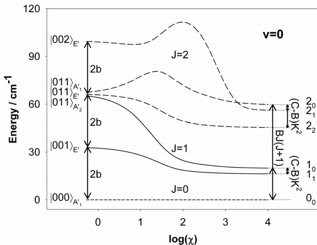
Figure 2.6. E_v = 0 energy level correlation for \text{XH}_3 J = 0, 1, 2 as function of intermolecular stiffness, \chi . For small \chi , the pattern reflects three freely rotating hydrogens, which for large \chi smoothly transitions into the rotational energy pattern characteristic of an oblate symmetric top.
