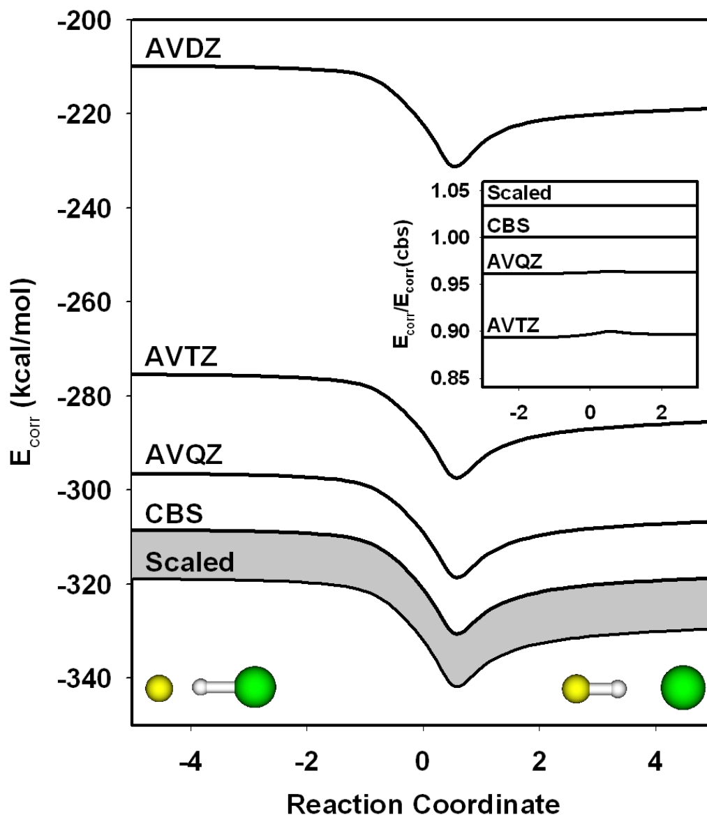
Figure 5.2: Correlation energy ( E_{\text{MRCI}} - E_{\text{MCSCF}} ) recovered for each basis set, AVnZ. - The nearly constant ratio of recovered correlation energy relative to the CBS extrapolation (see inset) illustrates how correlation scaling effectively mimics a larger active space.
