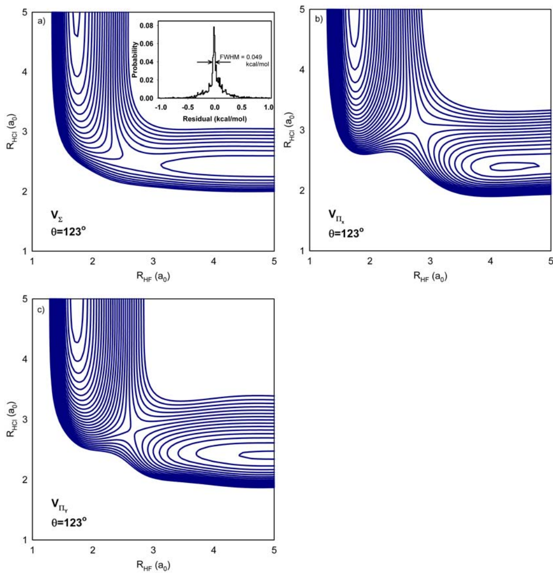
Figure 6.7: 2D contours (at \theta=123^\circ ) for the a) V_\Sigma , b) V_{\Pi_x} , and c) V_{\Pi_y} diabats with 3 kcal/mol spacing. A sample histogram of residuals for fitting the V_\Sigma function is also shown in a). The values are not distributed normally, which is why the RMS (0.34 kcal/mol) is considerably larger than the FWHM (0.049 kcal/mol).
