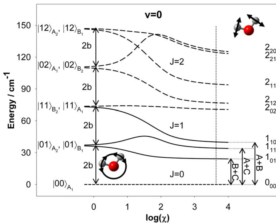
Fig 2.3. E_J = 0, 1, 2 energy level correlations for \text{XH}_2 in the ground vibrational state, plotted for the first few lowest energies versus potential stiffness, \chi . At small \chi , the energy separations reflect uncorrelated free rotation of the hydrogen atoms. At large \chi , however, this smoothly transitions into the characteristic J_{K_a K_c} patterns of a rigid asymmetric top.
