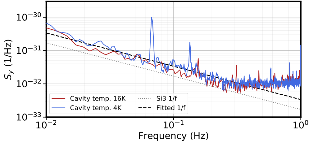
Figure 5.21: Residual noise S_{\text{residual}} + S_{\text{Brown}} after cancellation of the birefringent noise at both 4 K and 16 K shows no temperature dependence.
