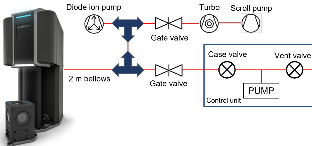
Figure 4.33: Schematic of the modifications for additional pumping on the cryostatation. Montana Instruments provides a control unit connected to the cryostatation with a long 2 m, 0.375" ID vacuum bellows. Within the control unit is a small roughing pump that is valved off from the bellows with a case valve contained within the control unit. A vent valve can be left open to the environment or connected to a nitrogen canister to vent the system to ambient pressure. We removed this connection by separating it from the pumping bellows with a gate valve. Instead, we add a tee that is connected to a turbo and scroll pump. After operating these two for a few days, we valve them off and activate a small 2 L/s diode pump.
