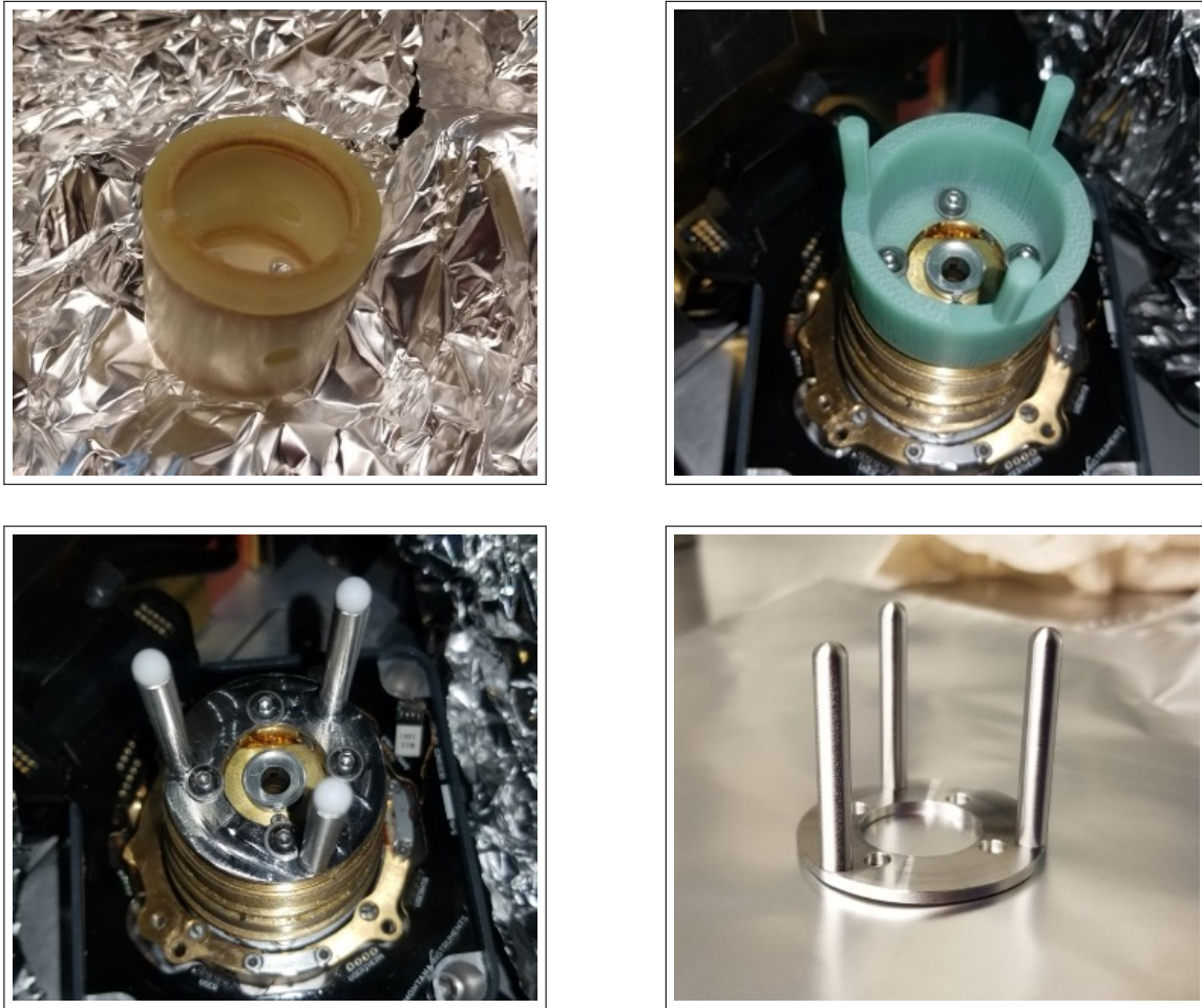
Figure 4.17: Various cavity mounts that we tested for improved sensitivity to acceleration noise. Top left: The original folded cup design from Si4, made from G10 composite. Top right: A simplified structure made from G10. Bottom left: A monolithic stainless steel support machined a block of 316 stainless. Hemispherical divots have been milled out from the top of each post. Spheres of different material can be placed within each divot, the image shows a set of teflon balls resting within the indentations. Bottom right: Our final cavity support made entirely from stainless steel
