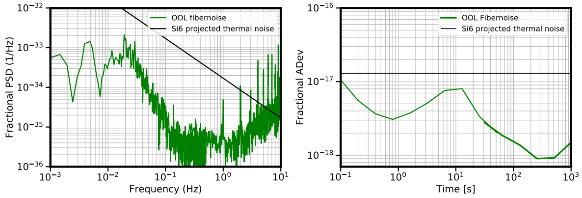
Figure 4.37: Measurement of the dissemination noise using the schematic shown in Fig.4.36. Left: Fractional frequency noise of the measurement. Right: Fractional Allan deviation of the measurement. Dissemination noise is well below the projected thermal noise limit of Si6.
