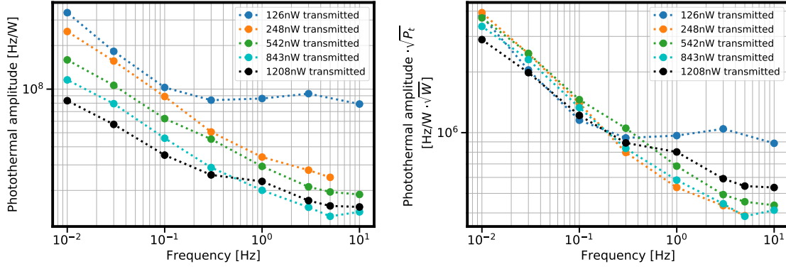
Figure 5.8: Left: Measured photothermal transfer function of the cavity response when modulating the transmitted power while locked to a single polarization mode of Si6. Data is taken at an operating temperature of 4 K. Right: Renormalizing the left set of curves by \sqrt{P_{transmitted}} .
