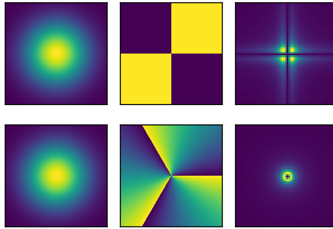
Figure 5.15: Generation of higher order modes with phase plates. The top row shows the phase plate (middle) needed for converting the fundamental mode (left) into the HG_{11} mode (intensity profile on the right). Yellow regions of the mode converter imprint an additional \pi phase shift when compared to the purple regions. The bottom row shows a similar procedure for generating the LG_{03} mode.
