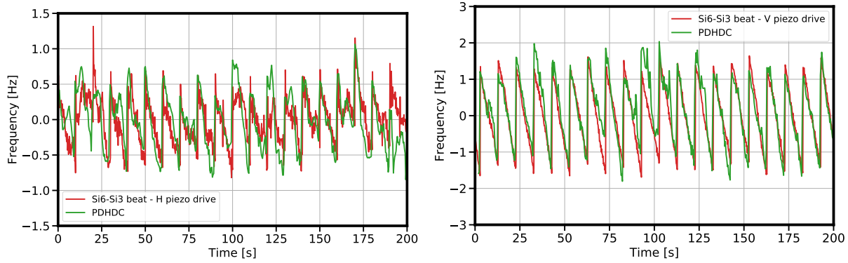
Figure 5.38: Modulating the voltage applied to the piezo allows us to measure a transfer function between the cavity frequency response and changes in the PDH DC signal. We do this for both axes to measure the system’s sensitivity to beam pointing. Left: The piezo is placed in the mirror’s horizontal pin. We drive it with a sawtooth and simultaneously record the frequency deviation. Red trace is the frequency response, and the green trace is the PDH DC voltage converted to frequency via our measured coupling. Right: Same data, except the piezo is now driving the mirror’s vertical pin.
