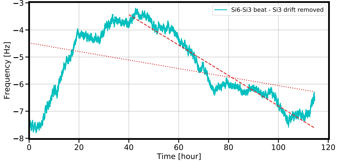
Figure 5.41: A five day measurement of the Si3-Si6 beatnote with the Si3 drift removed. During this period the Si3 drift was measured by the SrI lattice clock so its sign and magnitude is known. The dotted line is a fit to the entire dataset and finds a fractional drift rate of -2.3 \times 10^{-20}/\text{s} , whereas the dashed line fits to the latter two thirds where a more linear behaviour is observed. This segment finds a fractional drift rate of -5.6 \times 10^{-20}/\text{s} .
