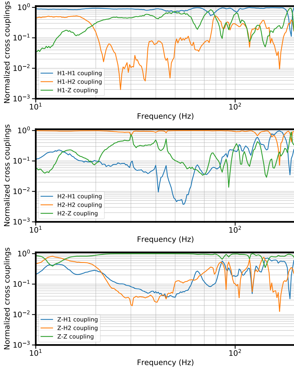
Figure 4.20: Plots of the coherent response measured along each axis when driving the AVI along one direction. In the top plot for example, the AVI is driven along H1 and we show the corresponding transfer functions a_i / \sqrt{\sum_i a_i^2} . The vast majority of the coherent displacement occurs along H1 at low frequency, though in regions around 50 Hz and 80 Hz, an equal response is measured in the vertical axis. Single axis feedback along H1 would exhibit strong cross coupling to another axis at these frequencies.
