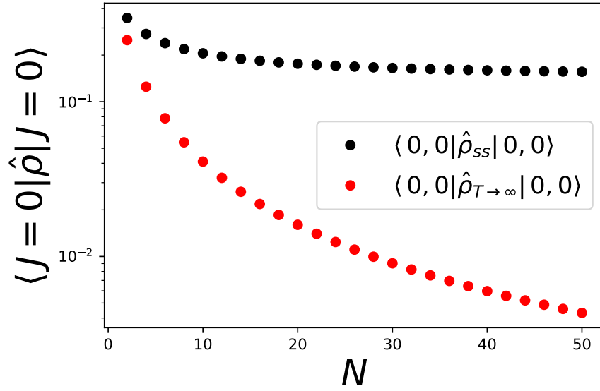
Figure 5.8: The population of the J = 0 state as a function of the atom number. The values of the superradiant lasing scheme (black dots) are given by the steady-state of Eq. (5.24), while the infinite temperature state values (red dots) are calculated by Eq. (5.19). The repump rate for each N is given by w = \Gamma_c/N .
