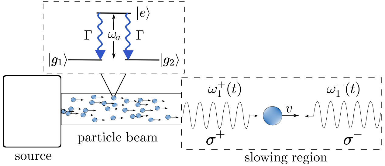
Figure 3.8: Particles exit an atom or molecule source and enter a slowing region. The spatial setup of the counterpropagating lasers, which have time-dependent frequencies \omega_1^-(t) and \omega_1^+(t) and polarizations \sigma^- and \sigma^+ for cycle 1, and a sample particle with velocity v in the laboratory frame are displayed in the slowing region. The circular inset shows the three-level internal structure of each particle.
