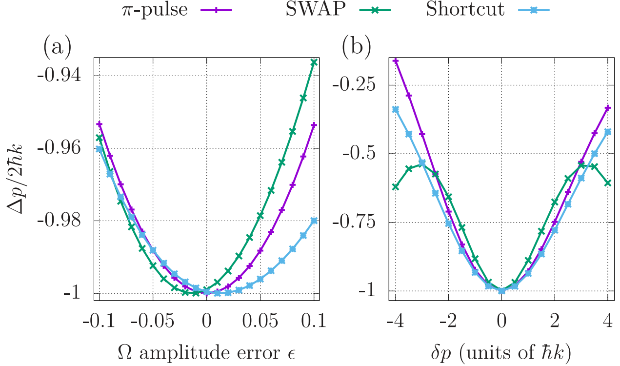
Figure 3.6: Robustness comparison of \pi -pulse slowing (purple, plus), SWAP slowing (green, cross), and the shortcut scheme (blue, circle with cross) over a \bar{p} \rightarrow \bar{p} - 2\hbar k transfer process. Ideally, the resulting impulse \Delta p satisfies \Delta p/2\hbar k = -1 . The evolution is purely coherent ( \Gamma = 0 ), the momentum of the particle (which is addressed by the laser frequencies) is \bar{p} = 2\hbar k , and the Rabi frequency is \Omega = 10\omega_r for all processes. (a) Impulse \Delta p experienced by the particle, in units of the ideal impulse magnitude 2\hbar k , as a function of the error in the Rabi frequency amplitude \epsilon [see Eq. (3.53)]. The shortcut scheme is the most robust protocol when \epsilon > 0 . (b) \Delta p/2\hbar k as a function of the relative momentum of the particle \delta p with respect to the momentum \bar{p} = 2\hbar k used in the laser frequencies [see Eqs. (3.1) and (3.54)]. For this set of parameters, the shortcut and \pi -pulse scheme are generally more robust than SWAP slowing. \pi -pulse parameters are: T = 0.314/\omega_r and \beta = \pi/2 . SWAP slowing parameters are: T = 1/\omega_r and \Delta_s = 50\omega_r . Shortcut parameters are: T = 0.44/\omega_r , \delta_{\text{cut}} = 230\omega_r , and \beta = 0.5\pi/2 .
