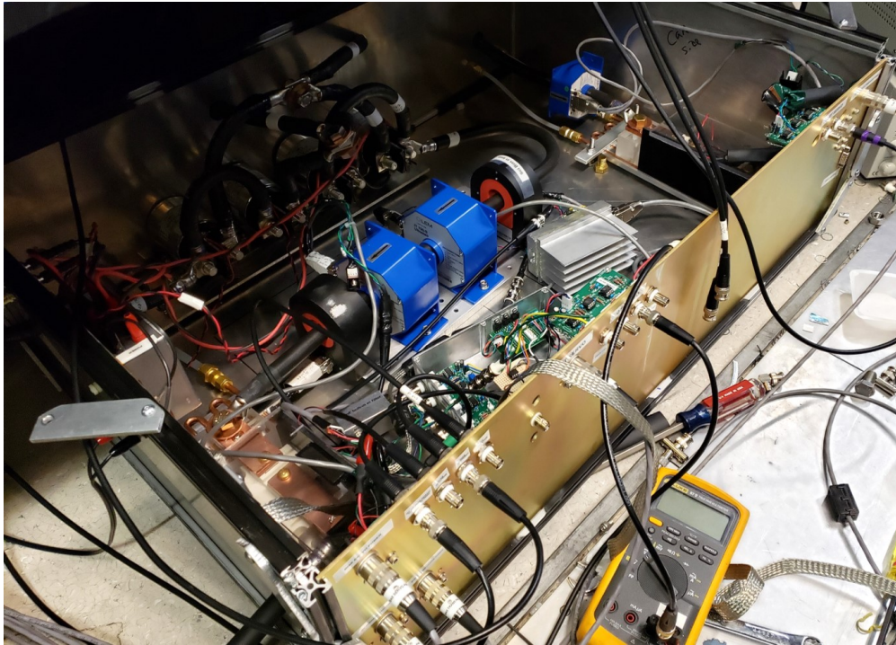
Figure 2.5: Magnetic field control enclosure. I constructed this enclosure as part of several efforts in our lab to reduce magnetic field noise. The box contains the H-bridge relays for the science coils in the rear of the box (upper left, difficult to see). It also contains the following for the cart coil circuit and the science coil circuit: current sensors, IGBTs, cooling plates for the IGBTs, servo electronics, sense resistors and their TECs, and inputs/outputs for water, analog and digital control, and finally power.
