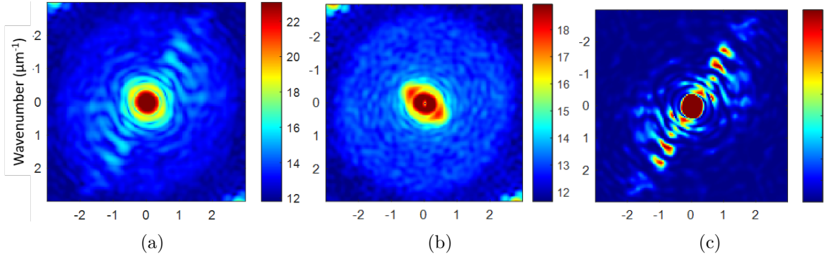
Figure 6.3: Squared FFT in the presence of atoms, x and y axes are wavenumbers k = 2\pi/\lambda in inverse microns. The color axis in (a,b) is \ln(S_{0_{raw}}) . The same region of real space is analyzed for each panel. In (a) the OD image for each individual experimental cycle (51 total images) was analyzed with no subtraction of the average. In (b) we do perform the subtraction of the mean OD prior to computing the FFT. In (c) the effect of subtracting the average is shown for the central region of Fourier space. To compute (c), the array values (without taking the log) in (b) are subtracted from (a) (also without taking the log) and divided (pixel-wise) by the values shown in (b). Therefore, (c) indicates the fractional increase in noise for each pixel in Fourier space if the average is not subtracted. Contrary to the case where no atoms were present shown in Fig. 6.2, subtraction of the mean density profile is required, as otherwise noise from the probe beam is written onto the atoms. In some regions of k -space the noise from probe beam may be more than 10x the atomic signal. Unlike in Fig. 6.2, we only show the resolved region, indicated clearly by the plateau reaching out to nearly k = 3 \mu\text{m}^{-1} in (b).
