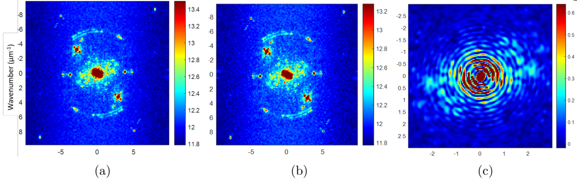
Figure 6.2: Squared FFT in the absence of atoms, x and y axes are wavenumbers k = 2\pi/\lambda in inverse microns. The color axis in (a,b) is \ln(S_{0_{raw}}) . The same region of real space is analyzed for each panel. In (a,b) no atoms were present and the logarithm is display for increased visibility. In (a) the OD image for each individual experimental cycle was analyzed with no subtraction of the average. In (b) we do perform the subtraction of the mean OD prior to computing the FFT. In (c) the effect of subtracting the average is shown for the central region of Fourier space. To compute (c), the array values (without taking the log) in (b) are subtracted from (a) (also without taking the log) and divided (pixel-wise) by the values shown in (a). Therefore, (c) indicates the fractional increase in noise for each pixel in Fourier space if the average is not subtracted; despite the visual similarity of (a) and (b), subtracting the mean OD suppresses noise on the order of 25% for k > 1 . In (a,b) the entire Fourier profile is shown; features at k > 3 are imaging artifacts well beyond our resolution.
