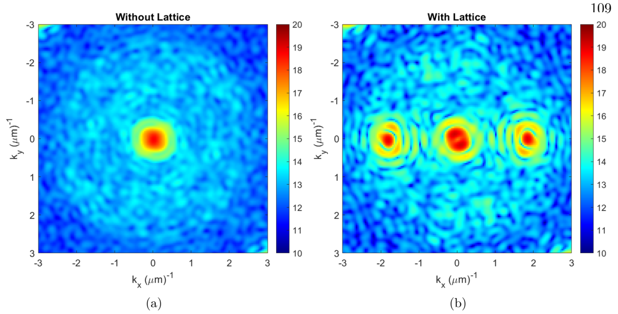
Figure 5.4: Averaged, squared Fourier transforms of the density with and without the X-lattice. The color scale is the same for both images, and the natural log of the squared Fourier transform is shown. Prior to computing the Fourier transform the average density profile in the absence of the lattice is subtracted from each individual cloud. On the left fifteen clouds without lattices were imaged, and no structure is apparent at k_x = 1.73\mu\text{m}^{-1} . In contrast, the presence of the lattice is apparent in (b). Only four density profiles are averaged in (b), making it slightly noisier.
