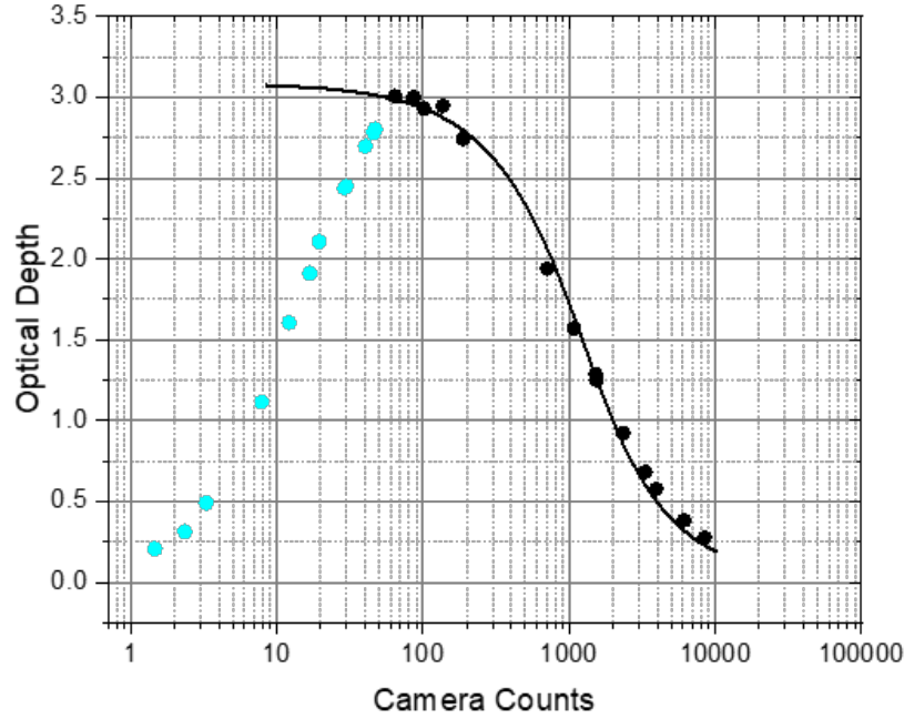
Figure 3.3: Optical density vs probe intensity. We fit to a model with the saturation intensity in counts is a parameter. Here the saturation intensity is found to be 602(22) counts for the 20 \mu\text{s} pulse. The cyan points are masked because the OD is washed out when signal to noise is low.
