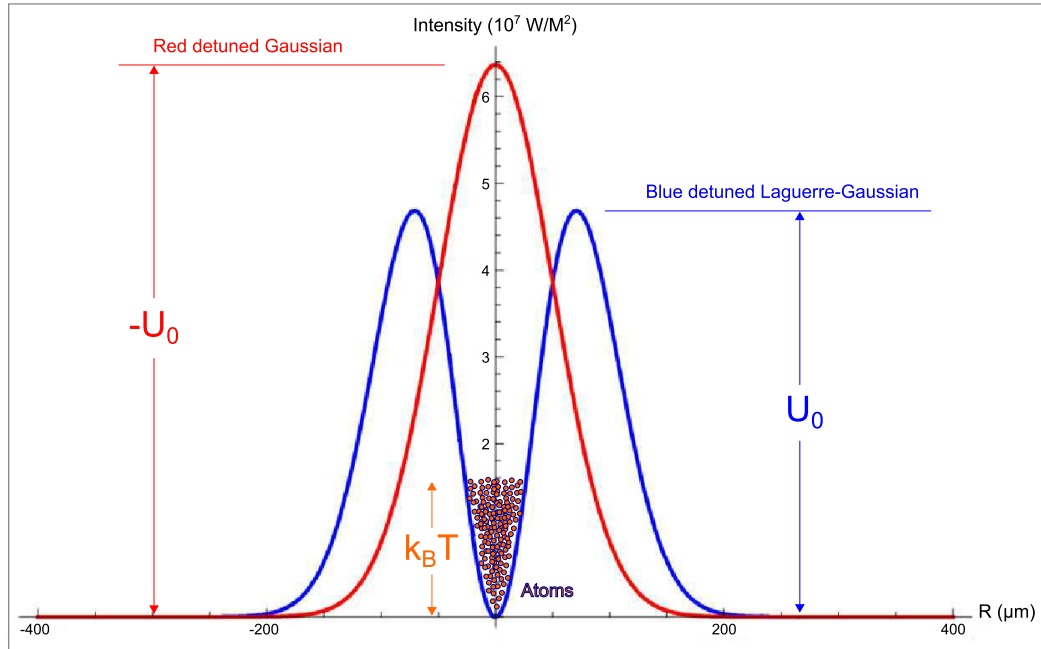
Figure 2.11: (Color) A plot of the potential of a red and blue detuned trap. The red detuned trap is a focused Gaussian beam with a waist of 100\ \mu\text{m} . The blue detuned trap is a focused Laguerre-Gaussian \text{TEM}_{01} mode with a 100\ \mu\text{m} waist and the same power as in the red detuned trap. In both cases atoms would be trapped in the center.
