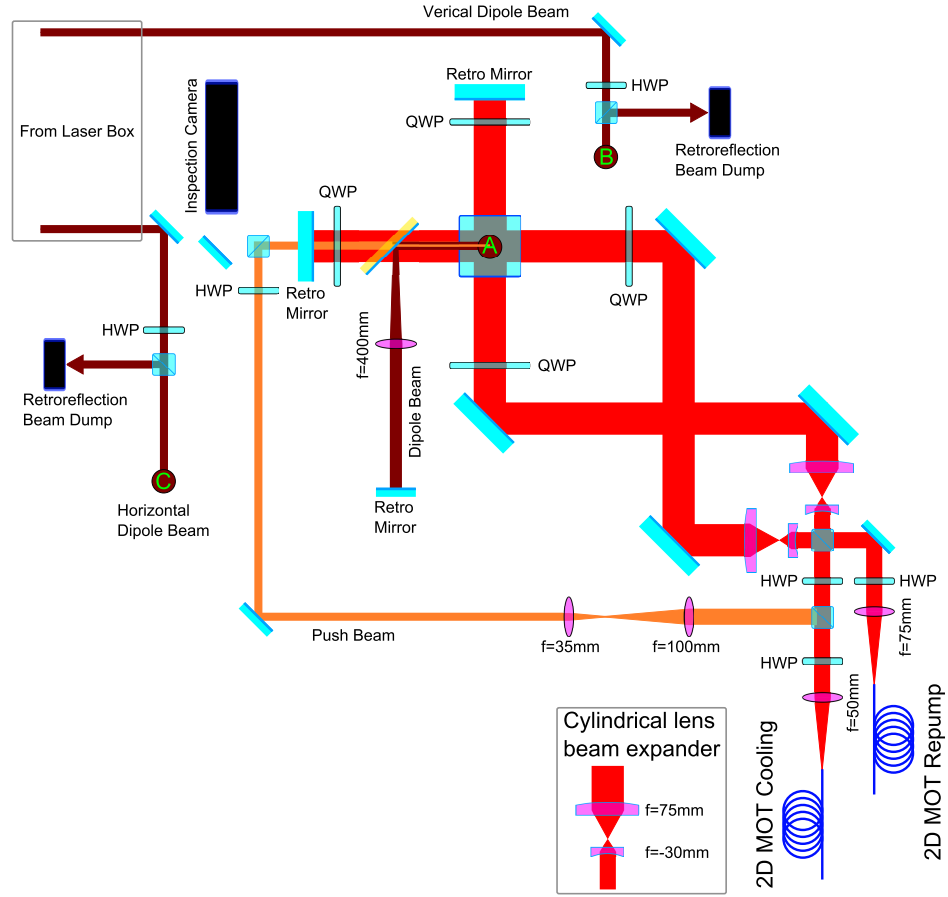
Figure 5.13: (Color) Tier 1 diagram of the vertical chamber setup, the 2D + MOT. The cooling fiber was collimated by an f=50\text{mm} achromat, with some light picked off for the push beam. The light was split and sent through a 2.5:1 cylindrical beam expander. A quarter waveplate made the light circularly polarized when it was sent into the cell and retroreflected. The push beam was shrunk in a 3:1 telescope and sent into the cell vertically. The dipole beams came from the laser box via free space on the left, where they were directed to tier 3 of the optical setup. The vertical dipole beam was sent upward at point B. The vertical dipole beam was sent downward from tier 3 through the cell, where it exited the cell at point A. The horizontal dipole beam was sent upward at point C.
