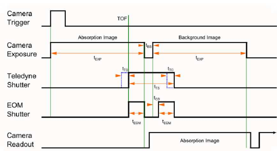
Figure 4.18: (Color) Diagram of the absorption imaging timing sequence in overlap mode. The camera is triggered before the TOF to be measured and begins exposing for a time t_{EXP} which is greater than the readout time of the camera. The absorption image is then taken so the falling edge of the probe pulse and camera coincide. Time t_{CD} , accounts for the delay the camera has from being triggered to the beginning of integration. An identical pulse to the first gives the background probe pulse, which is not resonant. The MEMS shutter closes shortly after the second pulse ends.
