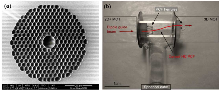
Figure 6.4: (Color) (a) Cleaved facet of the NKT HC-1060-02 hollow core photonic crystal fiber for 1060 nm. At the center is the 10\text{ }\mu\text{m} hollow core where a red detuned 1064 nm dipole beam would guide atoms with a mode field diameter of 7.5\text{ }\mu\text{m} . (b) Photo of the partially assembled PCF atom transport test cell. The 2\text{D}^+ MOT cell is on the left, where the atom source is located. The dipole guide beam is coupled through the 2\text{D}^+ MOT cell, and guides atoms through the connecting T-shaped chamber where they can be captured in a 3D MOT, a dipole trap, or detected, on the right.
