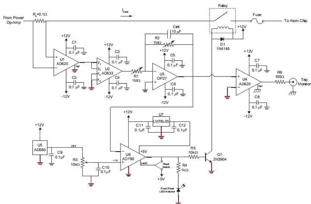
Figure A.4: Bipolar chip driver protection circuit diagram.
