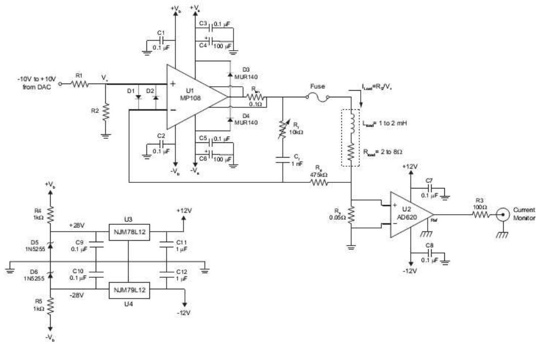
Figure A.2: Bipolar coil driver circuit diagram.
