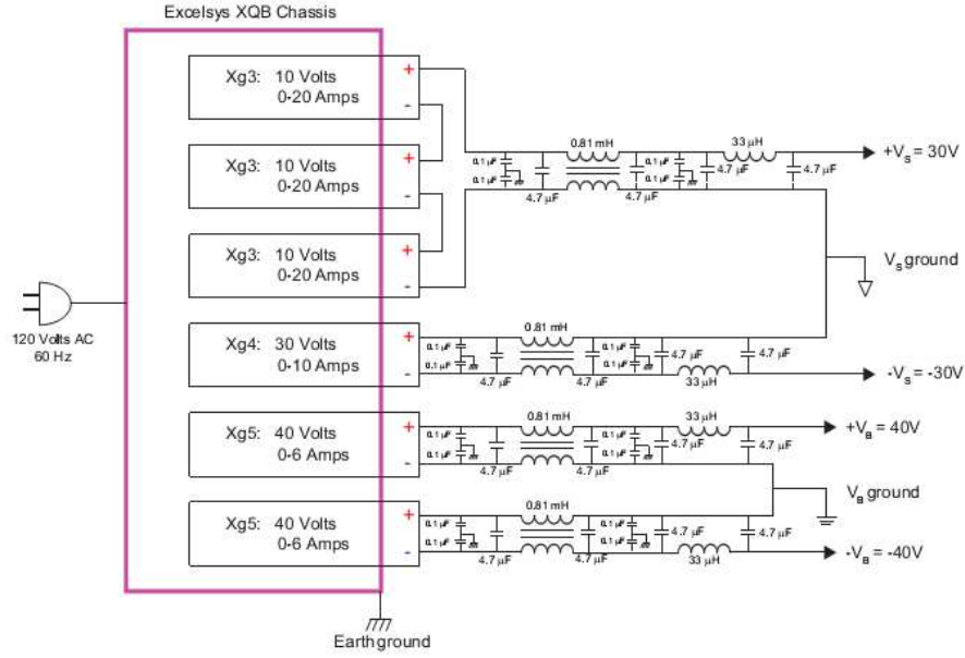
(a) Coil driver Excelsys power supply configuration.
