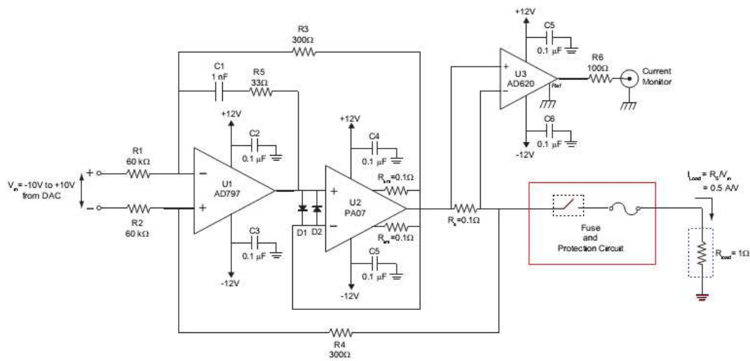
Figure A.3: Bipolar chip driver circuit diagram.
