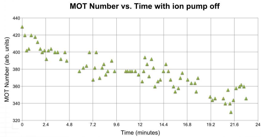
Figure 3.17: (Color) Plot of the MOT number vs. time without operating the ion pump. The MOT atom number decays by 17% over 24 min.
