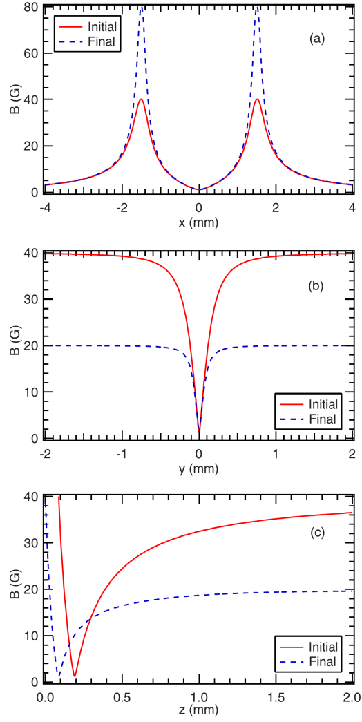
Figure 4.25: (Color) Plots of a chip H-wire scheme for forced direct evaporation in a magnetic trap. The magnetic field in the x-, y-, and z-dimensions are shown in (a), (b), and (c), respectively. The solid red line indicates the initial trap with parameters I_0 = I_h = 4 A, B_{0x} = 0 G, and B_{0y} = 40 G. The dashed blue line indicates the final trap with parameters I_0 = 1 A, I_h = 4 A, B_{0x} = 0.64 G, and B_{0y} = 20 G. Image credit [81].
