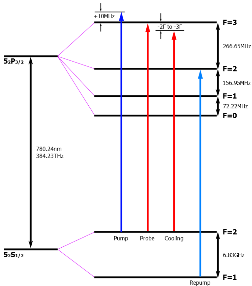
Figure 4.5: (Color) The ^{87}\text{Rb} D2 spectral lines and experimental laser frequencies.
