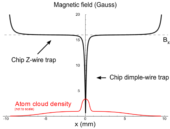
Figure 4.22: (Color) Plot of the RF evaporation chip dimple magnetic trap. The chip Z-wire trap is the plateau that extends from -10 mm to 10 mm along the x-direction, with a trap bottom of B_x = 16 G and trap top of B_x = 40 G. The dimple trap can be seen in the middle, with a trap bottom of 2 G and an effective trap top of B_x = 16 G. A representation of the atom cloud distribution is shown in red.
