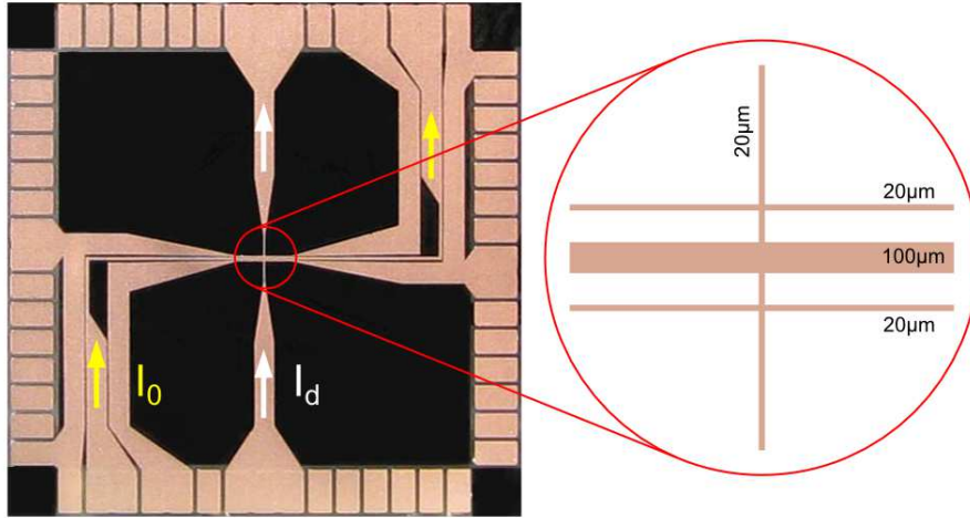
Figure 3.7: (Color) A photo of the atom chip designed for direct evaporation. There are three main traces, one with a 100\text{ }\mu\text{m} width and two that run parallel to it with a 20\text{ }\mu\text{m} width. There is one dimple trace that runs down the middle of the chip, which tapers to a 20\text{ }\mu\text{m} width at the center of the chip where it crosses the main wires.
