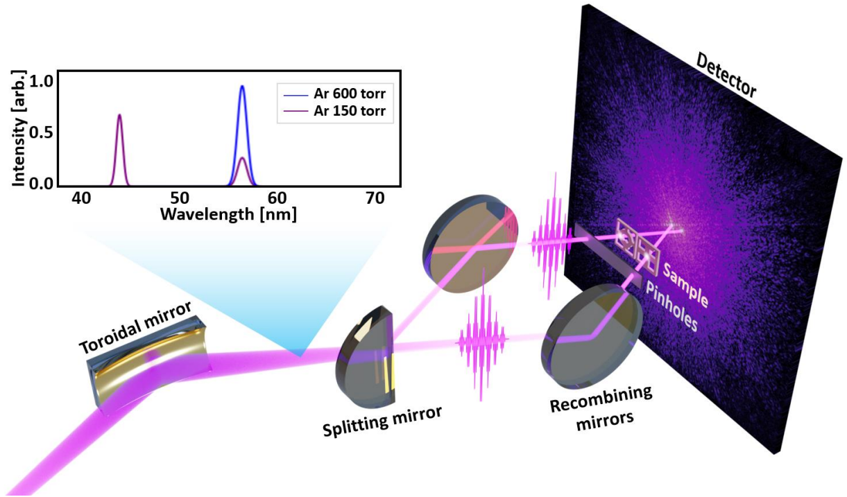
Figure 2.1: Schematic of the temporally multiplexed EUV microscope. The output of an HHG light source is divided into two separate paths and focused onto distinct areas of a sample, and the combined diffraction is recorded. Due to differences in the path lengths of the two beams relative to the extremely short duration of the HHG pulse train, the component diffraction patterns add incoherently, and the data can be directly used for multimode ptychography reconstructions. The insert shows the estimated spectra of the EUV light source. By adjusting the argon gas pressure in the waveguide, the generating conditions can be adjusted to select either a single harmonic peak at 56 nm, or two peaks at 44 nm and 56 nm. Figure adapted from [87].
