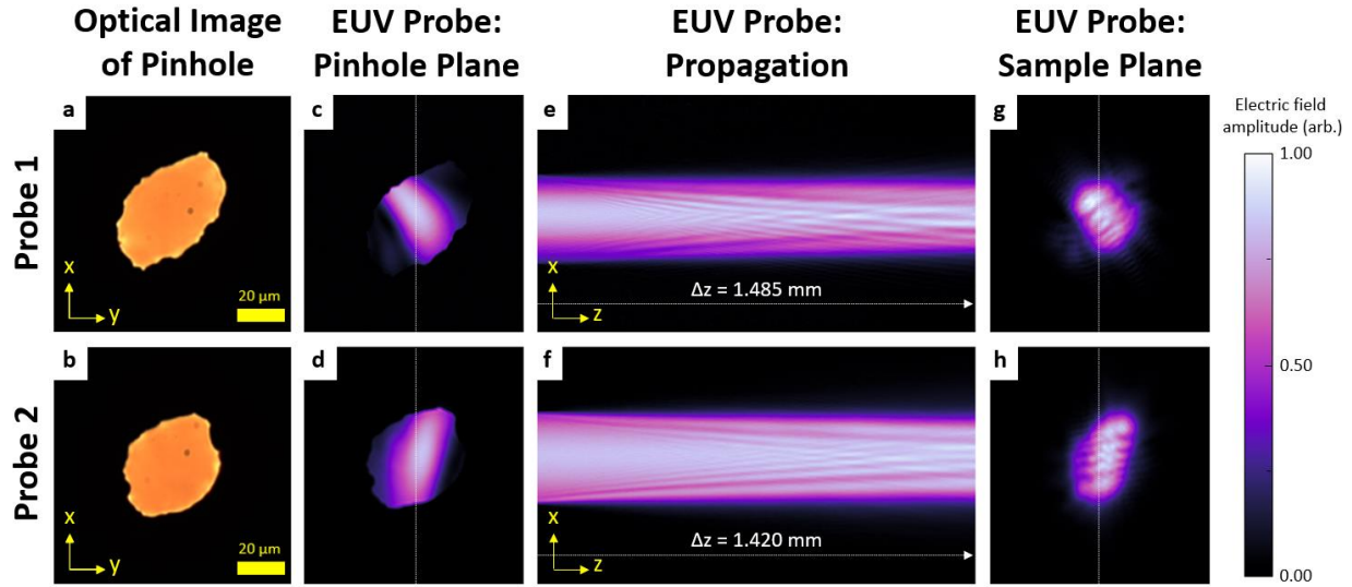
Figure 2.3: Characterization of reconstructed probes from multibeam ptychography scans. (a,b) Optical microscope images of the laser-drilled pinholes used to improve and constrain the two illuminating EUV modes for the ptychography microscope. (c,d) Reconstructed probes from the multibeam ptychography in the pinhole plane (c, probe 1; d, probe 2) (e,f) Evolution of the beams throughout propagation from the pinhole to the sample plane, shown as a slice at y = 0 , i.e., the vertical dashed white lines in c, d, g and h. (g,h) Reconstructed probes in the sample plane. Figure adapted from [87].
