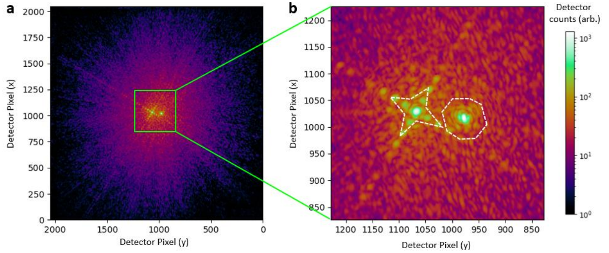
Figure 2.7: Diffraction pattern from two temporally incoherent illuminating modes. (a) Full detector area, showing two slightly separated DC peaks with overlapping diffraction orders out to the edges of the detector. (b) Close-up of the central part of the detector. The white dashed curves indicate the areas where the Fourier amplitude limit is applied to help decouple the two probe modes. Figure adapted from [87].
