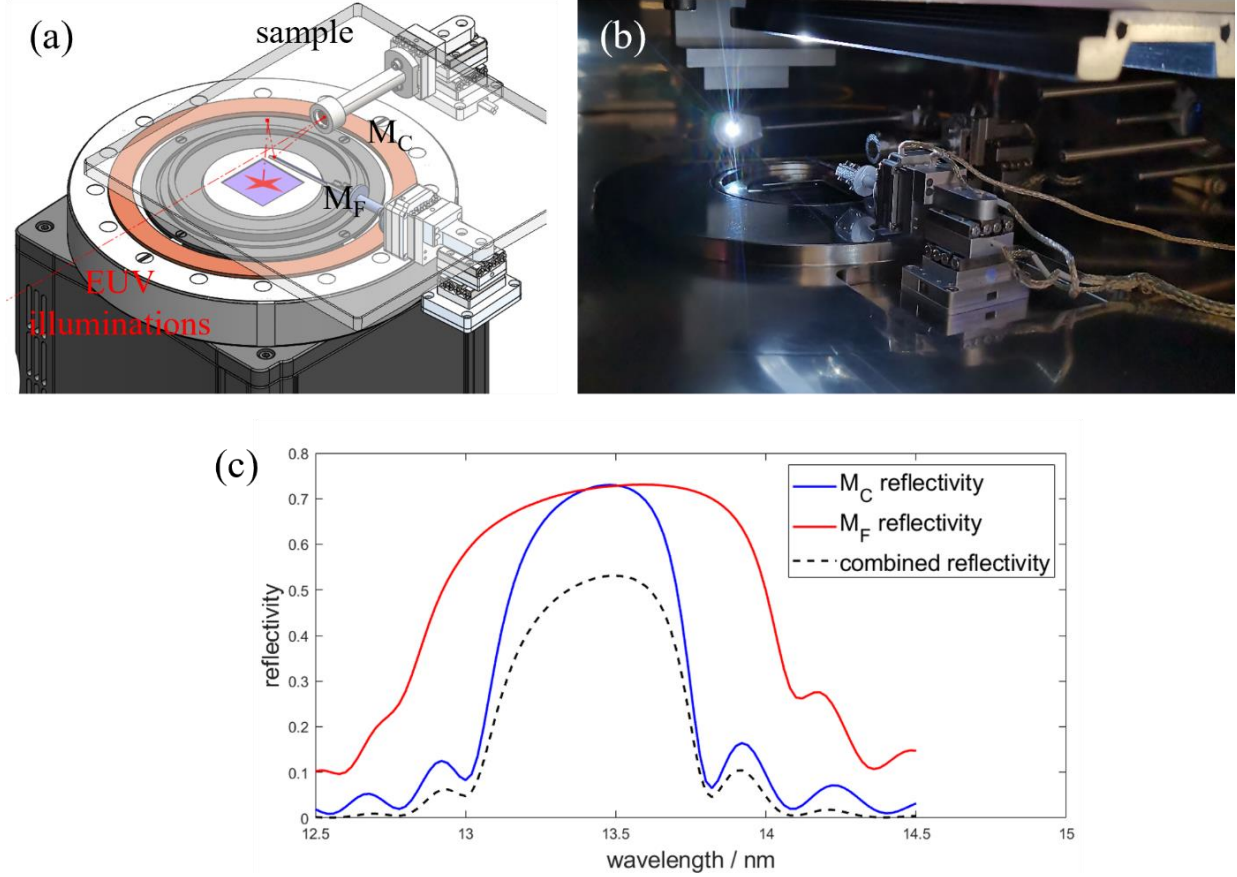
Figure 3.4: The lensless EUV microscope consists of two Si/Mo multilayer mirrors, M_C and M_F , to select out a single wavelength at 13.5 nm wavelength and focus it onto the EUV photomask sample at a 6^\circ angle of incidence from normal. The EUV beam reflects and diffracts off the sample and is collected by an EUV-CCD camera. (a) A schematic diagram and (b) a photo of the lensless EUV microscope. (c) The reflectivity vs wavelength curves for M_C , in blue, M_F , in red, and both mirrors, in dashed black.
