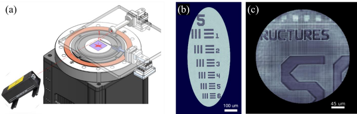
Figure 3.10: TEAMS system calibration and demonstration using visible lasers. (a) A schematic shows the coupling of a visible laser to the lensless imaging end-station for troubleshooting and preliminary demonstrations. (b) The amplitude of a ptychographic reconstruction of a 1951 USAF test target taken with a He-Ne laser at 632nm wavelength, showing excellent image quality and a spatial resolution of at least 17.54μm (element 6 in group 5), while the diffraction-limited spatial resolution is 7.31μm. (c) the amplitude of a ptychographic reconstruction of a semiconductor test sample from imec taken with a diode laser at 450nm wavelength.
