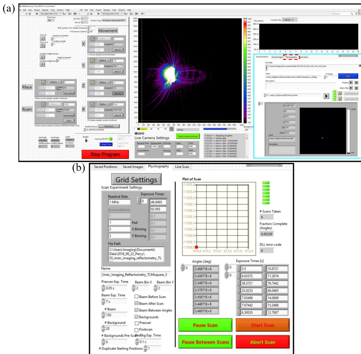
Figure 3.5: Screenshots showing the TEAMS data taking software user interface. (a) This screenshot shows the TEAMS data acquisition software full program. The functionality to setup and execute ptychography scans are under the “Ptychography” tab marked by the red dashed box within the cyan-highlighted area, of which a close view is shown in (b) .
