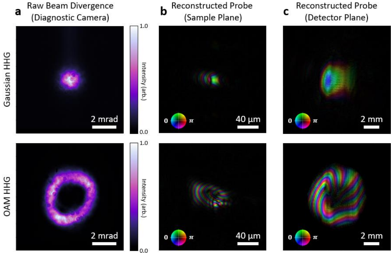
Figure 4.10: Gaussian and OAM HHG beam profiles in different planes. (a) Intensity profiles of the Gaussian and OAM HHG beams 1.5m after they are generated without focusing/defocusing optics in the middle. They are directly measured on a diagnostic camera. (b) The reconstructed Gaussian and OAM HHG beams in the sample plane. The beams are focused by a double-toroid system onto the sample. The intensity and phase are encoded in brightness and hue, respectively. (c) The reconstructed Gaussian and OAM HHG beams in the detector plane.
