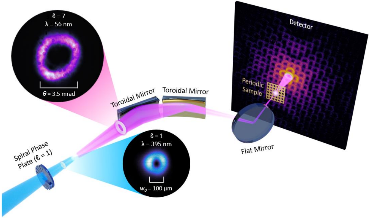
Figure 4.5: Schematic diagram of the experimental set-up for ptychographic imaging of highly periodic structures. A quasimonochromatic beam at \sim 56 \text{ nm} wavelength (either with a Gaussian mode or carrying OAM \ell=7 ) is generated via HHG. It is then focused by a double-toroid system onto the periodic structures to produce characteristic far-field diffraction patterns.
