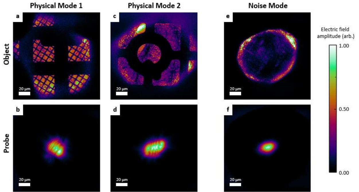
Figure 2.6: Physical and noise modes of the temporal multiplexing experiment. (a) Object 1 reconstruction at 56 nm, (b) Probe 1 reconstruction, (c) Object 2 reconstruction, (d) Probe 2 reconstruction, all shown in amplitude and corresponding to physical modes in the system. (e) Noise object 1 and (f) noise probe 1, accounting for decoherence effects in the system. Figure adapted from [87].
